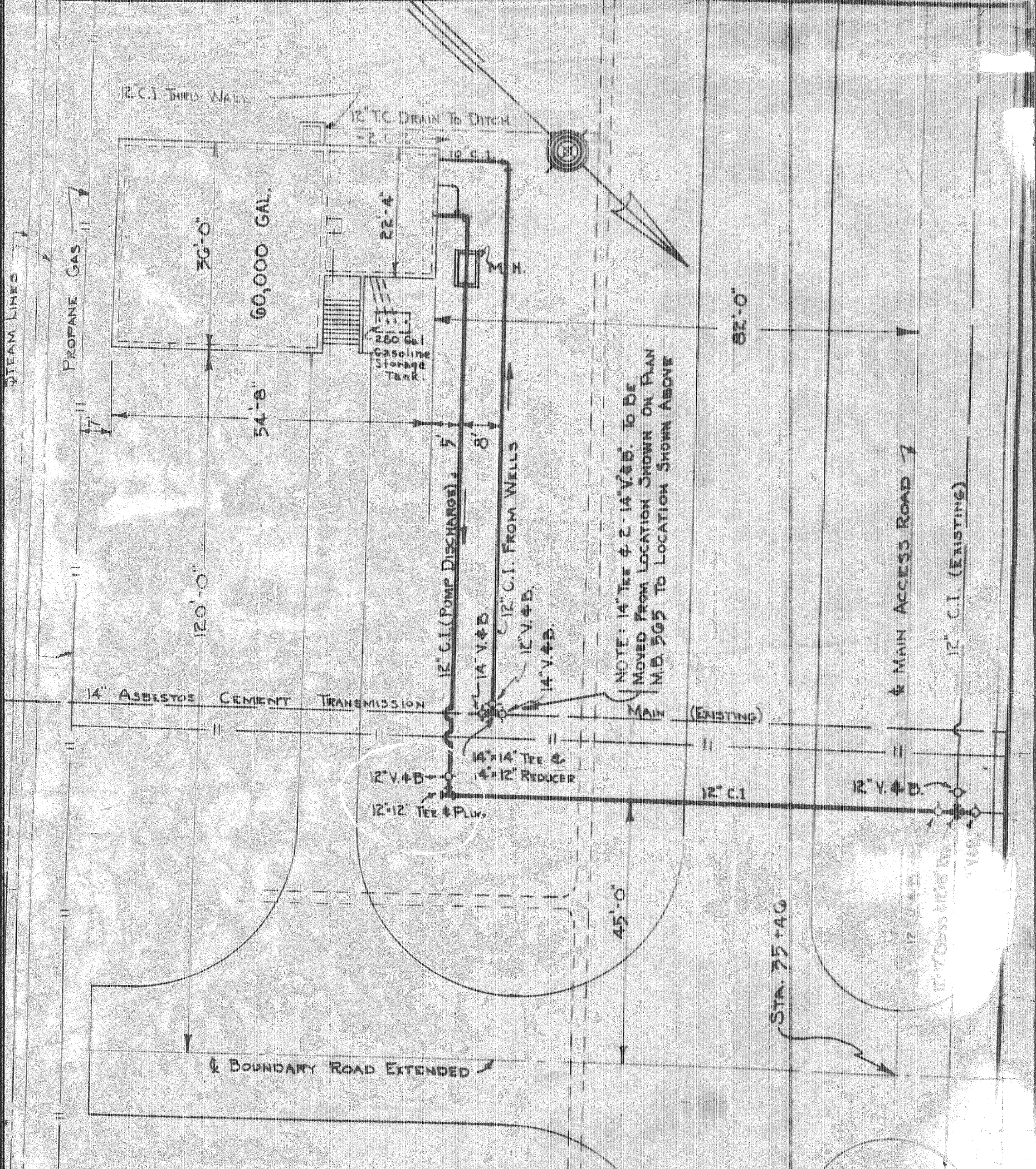
LOCATION PLAN. SCALE 1" = 20'
