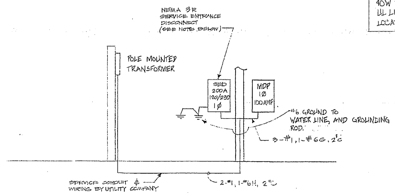
ELECTRICAL RISER NTS
