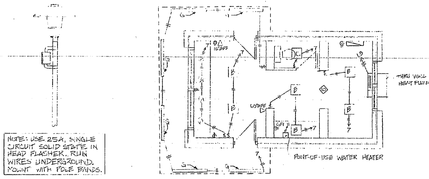
ELECTRICAL PLAN 1/4" = 1'-0"
