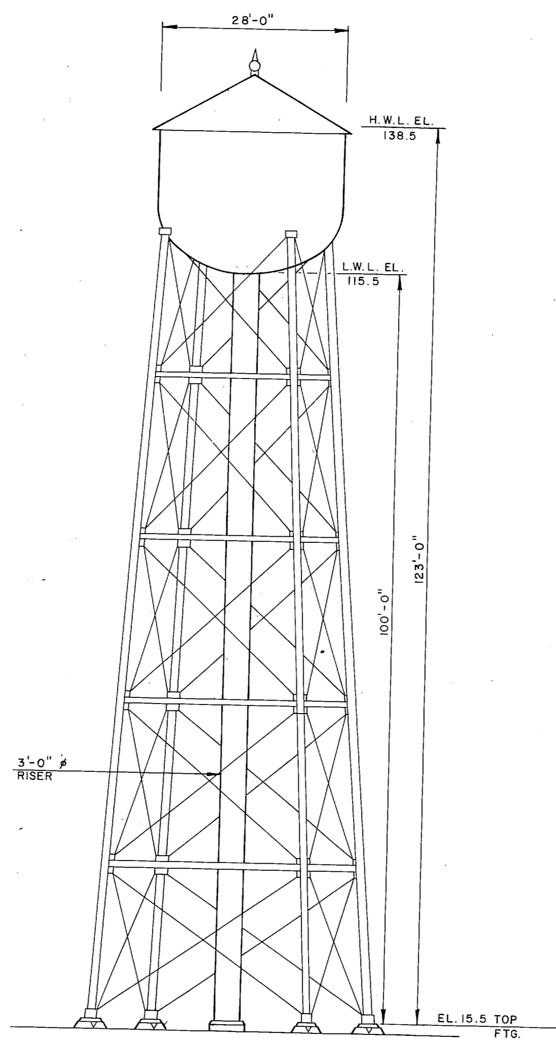
TANK S-BB-25 COURTHOUSE BAY 100,000 GAL.
