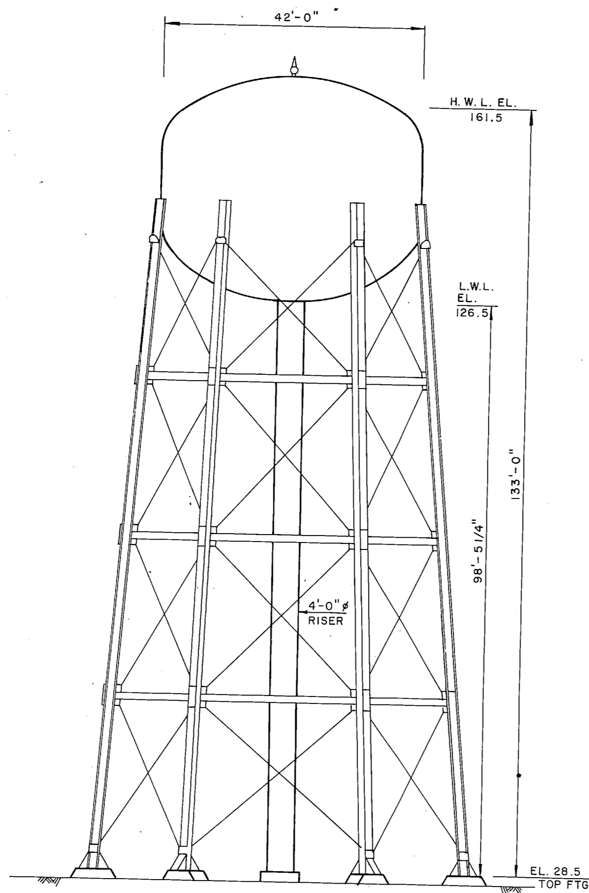
TANK S-29 HADNOT POINT 300,000 GAL.
