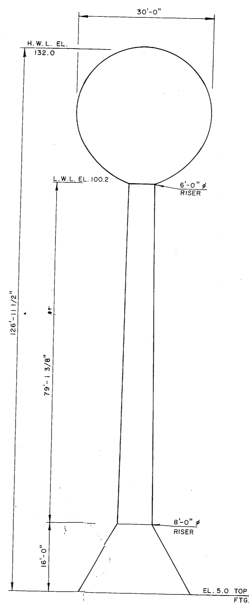
TANK S-BA-108 ONSLOW BEACH 100,000 GAL.
