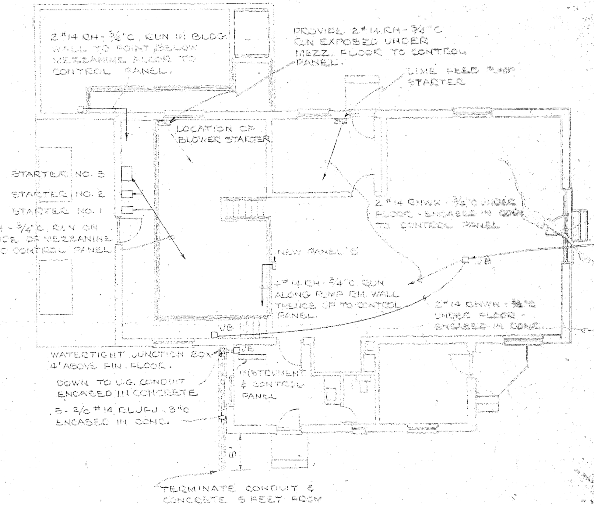
FLOOR PLAN SHOWING TELEMETRING CIRCUITRY
