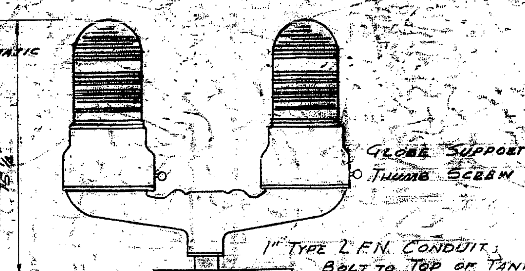
OBSTRUCTION LIGHT ON TOP OF TANK DOUBLE BULB WITH OBSTRUCTION LIGHT TYPE MULTIBULB CONDUIT WITH BULB GLOBS, IN ACCORDANCE WITH TECHNICAL SPECIFICATIONS 311-4-100
