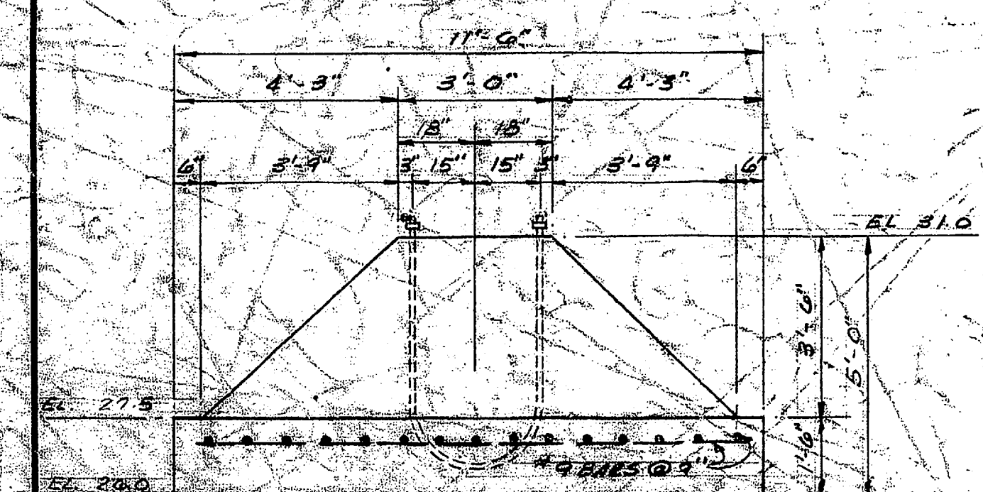
ELEVATION FOOTING SCALE 1/8" = 1'-0"
