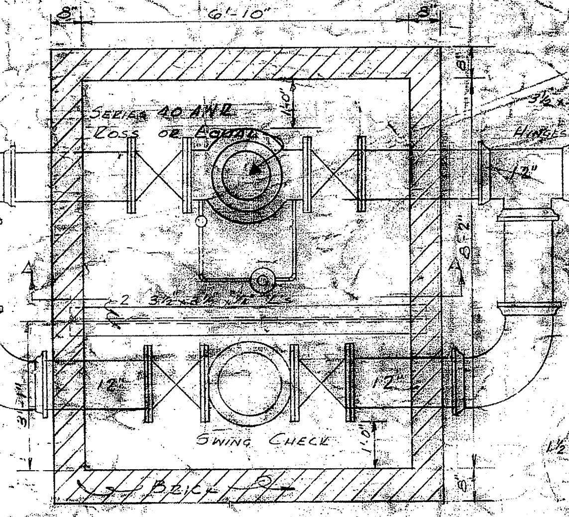
ALTITUDE VALVE BOX & BY-PASS SCALE 1/2" = 1'-0"
