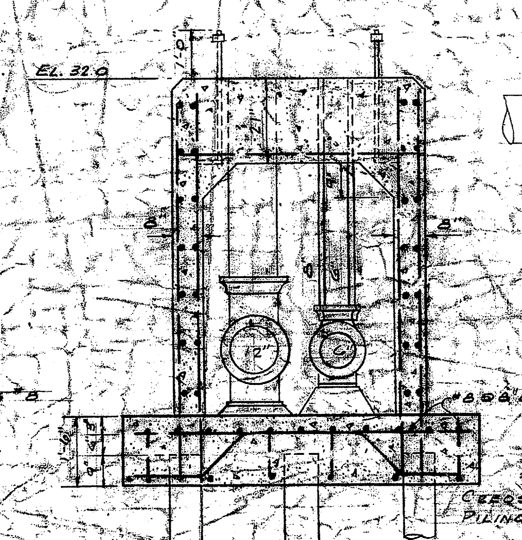
SECTION A-A SCALE 1/4" = 1'-0"
