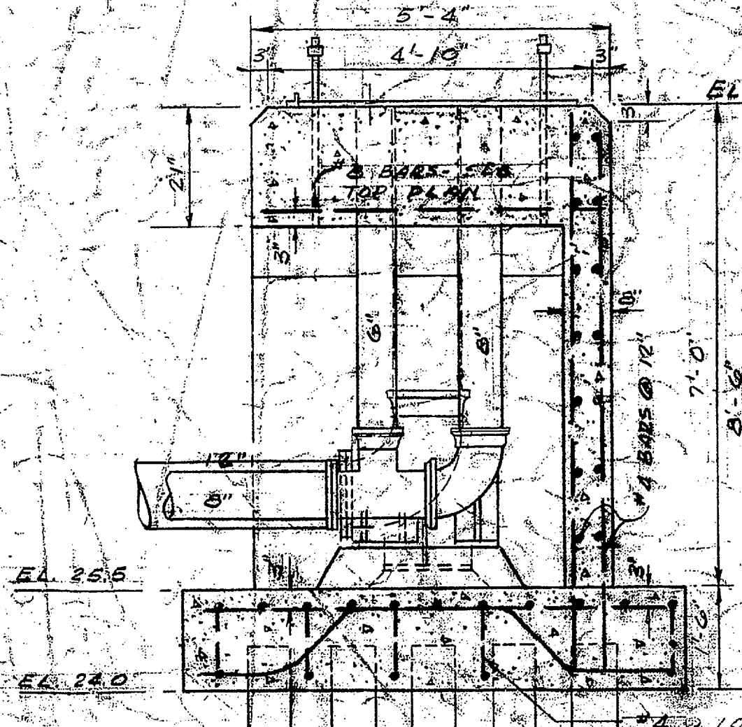
SECTION B-B SCALE 1/4" = 1'-0"
