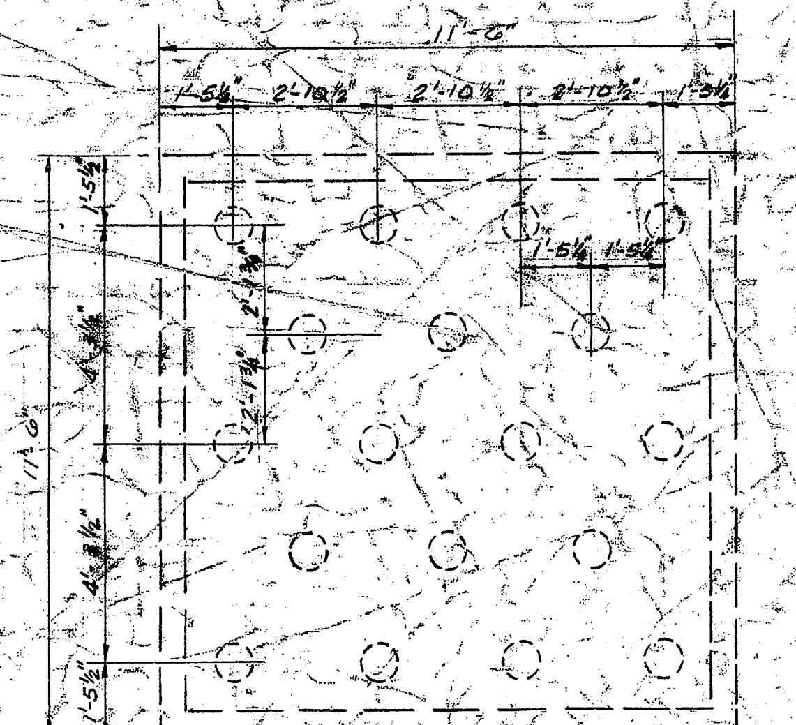
PILING PLAN FOR FOOTINGS SCALE 1/8" = 1'-0"
