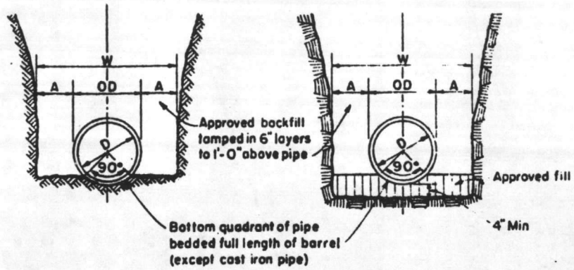
TRENCH IN EARTH
