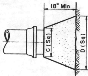
PLAN & ELEVATION PLUGS
