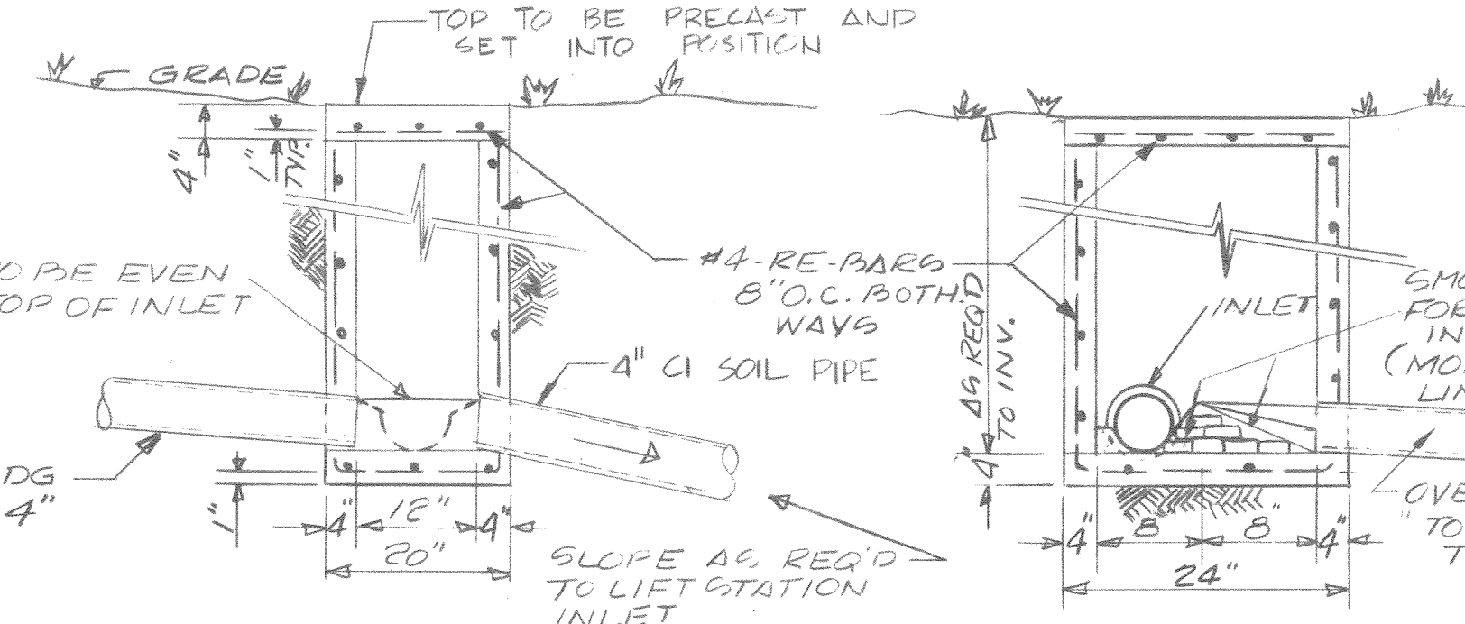
DETAIL "A" BUILDING STUB-OUT (NTS)
