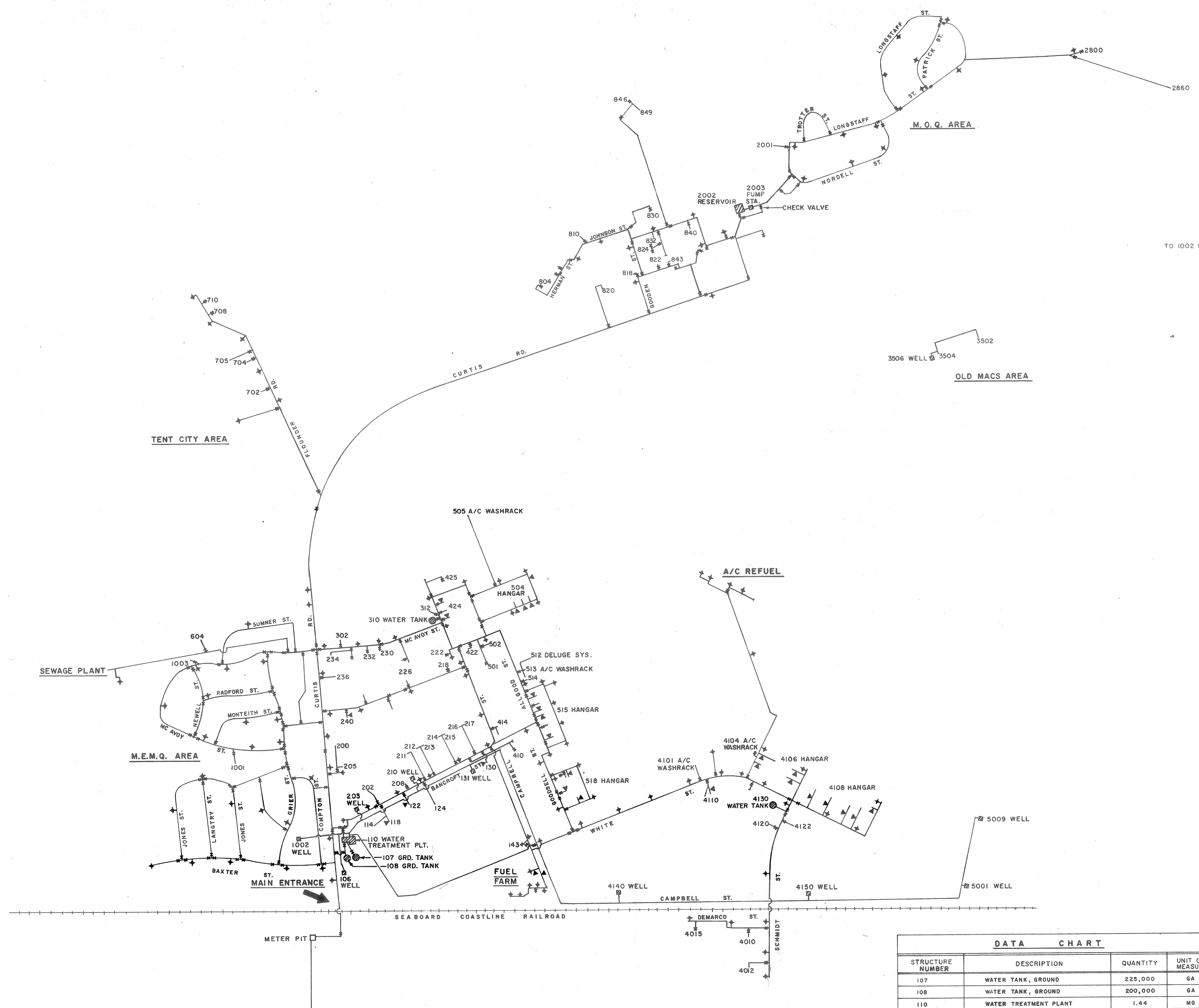
DISTRIBUTION SYSTEM - SCHEMATIC SCALE: 1" = 500'
