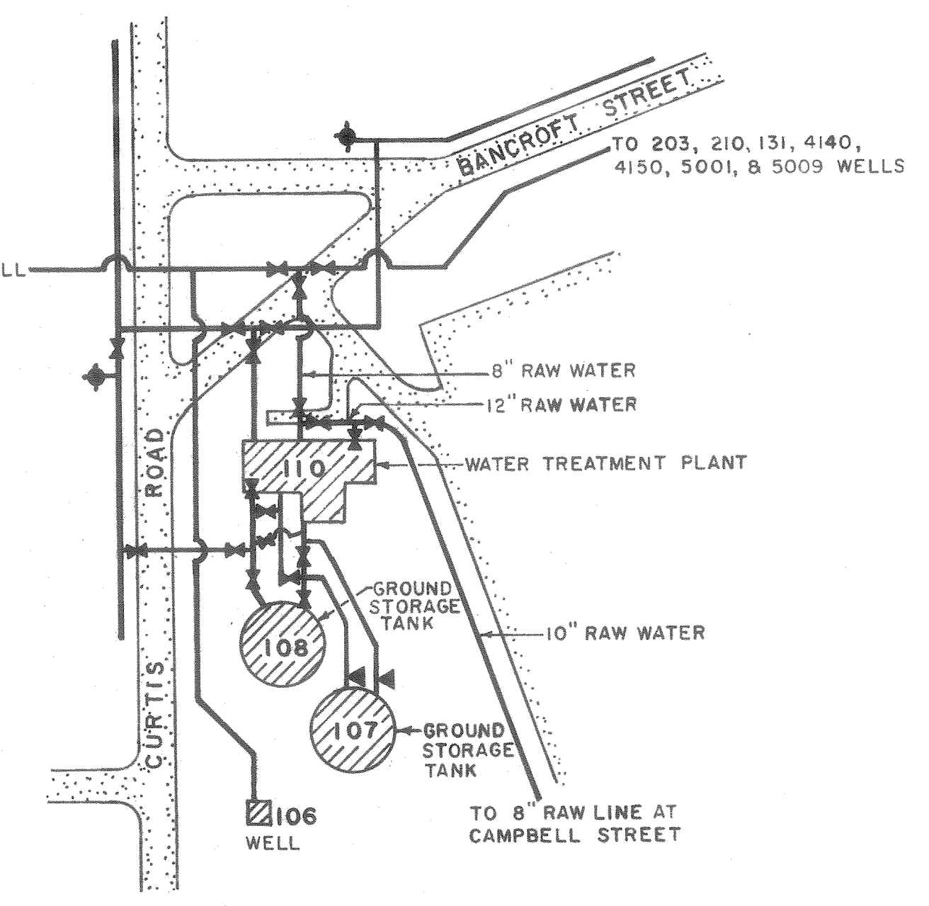
WATER PLANT AREA SCALE: NONE
