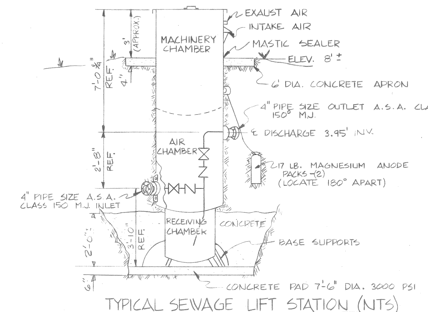
TYPICAL SEWAGE LIFT STATION (NTS)
