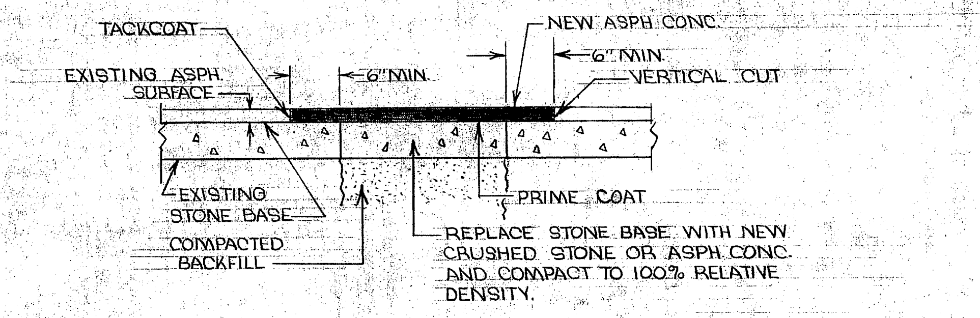
TYPICAL SECTION FOR REPAIR TO ASPHALTIC CONCRETE SCALE: N.T.S.
