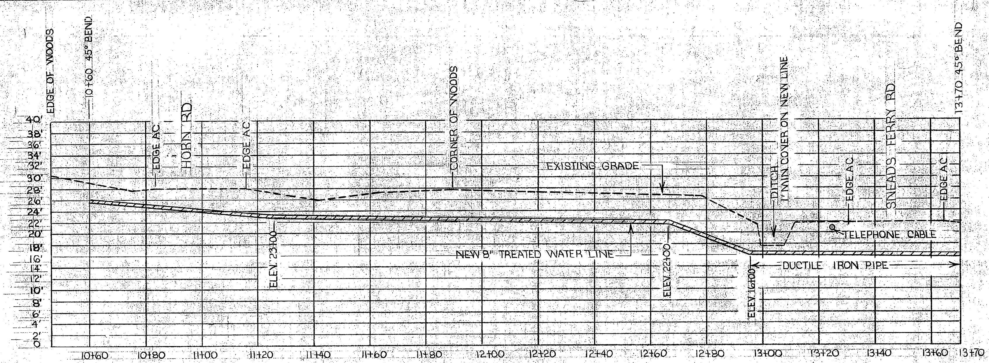
PROFILE OF HORN ROAD - SNEADS FERRY ROAD INTERSECTION SCALE: 1"=10'-0" VERTICAL 1"=20'-0" HORIZONTAL
