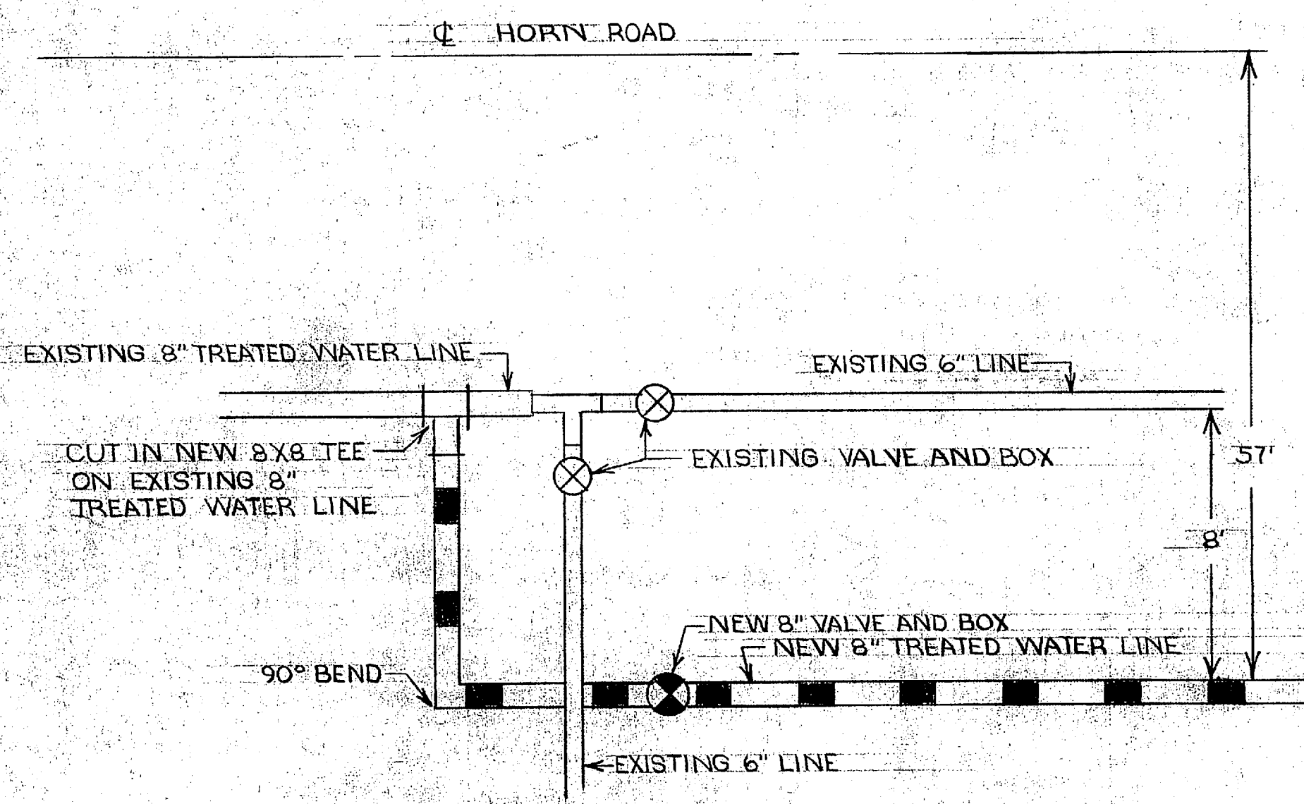
DETAIL #1 SHOWING TIE-IN FOR NEW 8" LINE TO EXISTING 6" TREATED WATER LINE SCALE: N.T.S.
