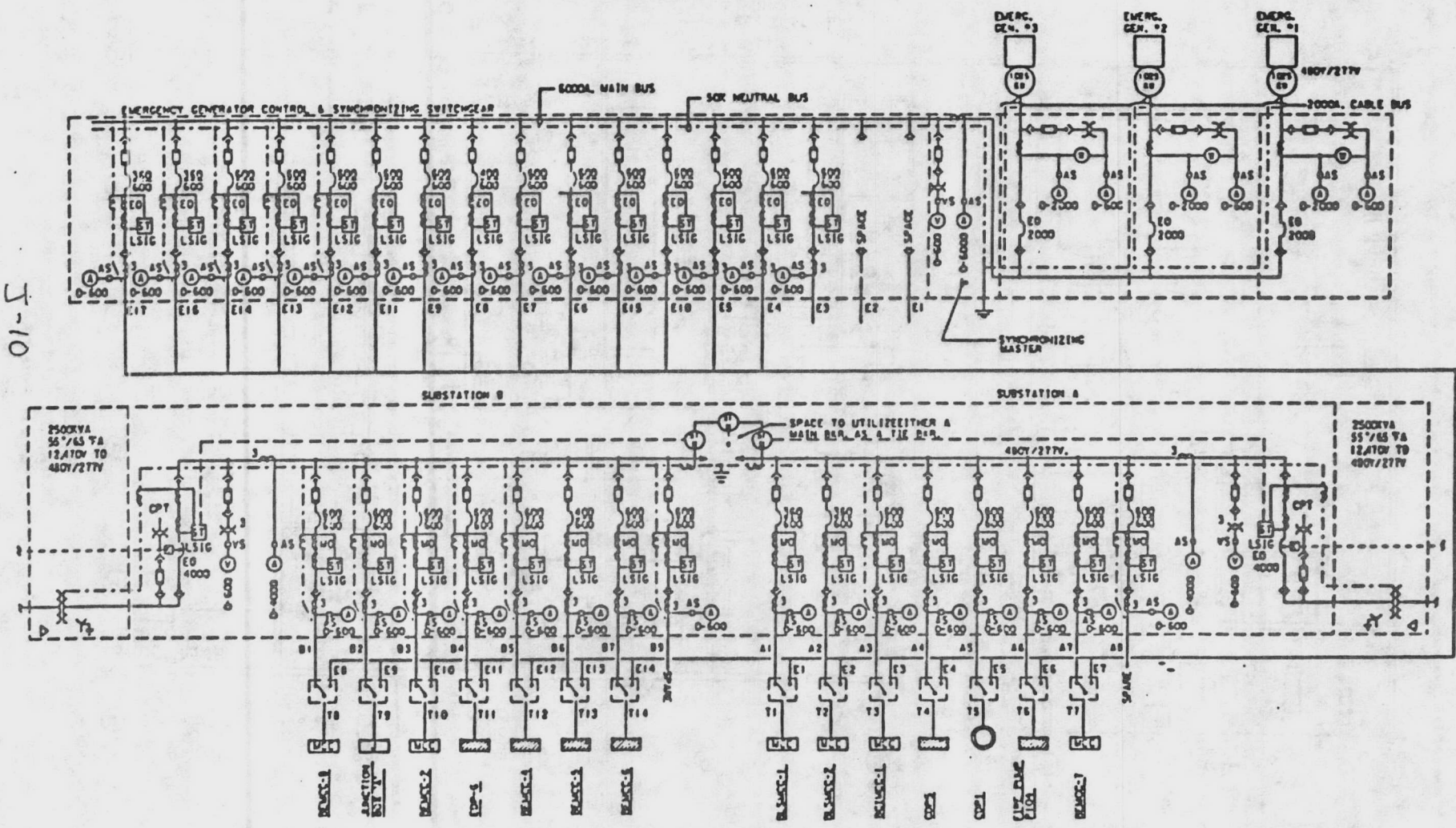
ESSENTIAL LOW VOLTAGE POWER SYSTEM SINGLE LINE DIAGRAM
