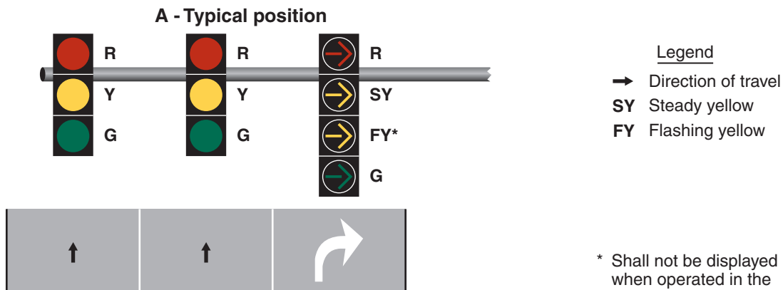
Figure 4D-19. Typical Position and Arrangements of Separate Signal Faces with Flashing Yellow Arrow for Protected/Permissive Mode and Protected Only Mode Right Turns
