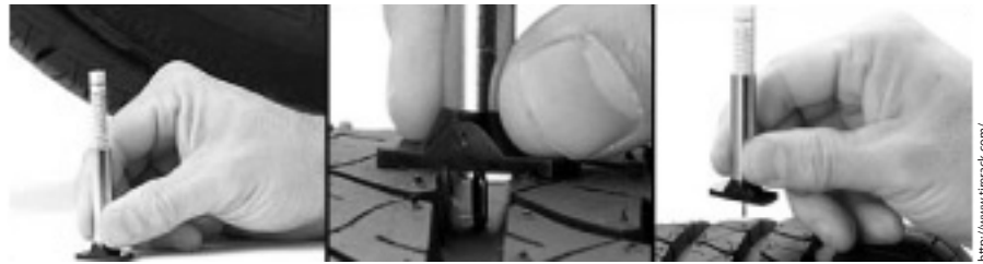
Left, to use a tire depth gauge, start by zeroing-out your gauge. Center, insert the gauge into a circumferential tire tread and press down. Right, read the gauge and record the tire depth. See detailed steps below.
