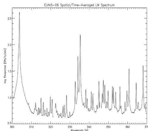
Spectral data from the EUNIS-06 mission, 36.203 NS, flown April 12, 2006.
