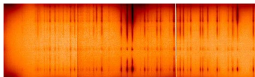
Spectral data from the EUNIS-06 mission, 36.203 NS, flown April 12, 2006.
