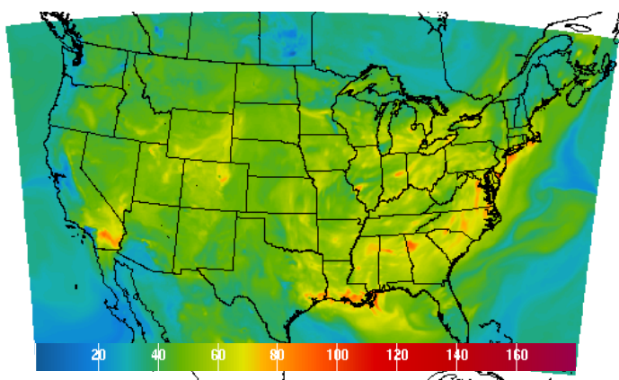
NOAA Sample operational air quality forecast guidance. Predicted ground-level ozone concentrations, (averaged over 8 hours, in parts per billion) show unhealthy levels of ground-level ozone in warmer colors (orange, red). Current predictions available at: www.weather.gov/qa
