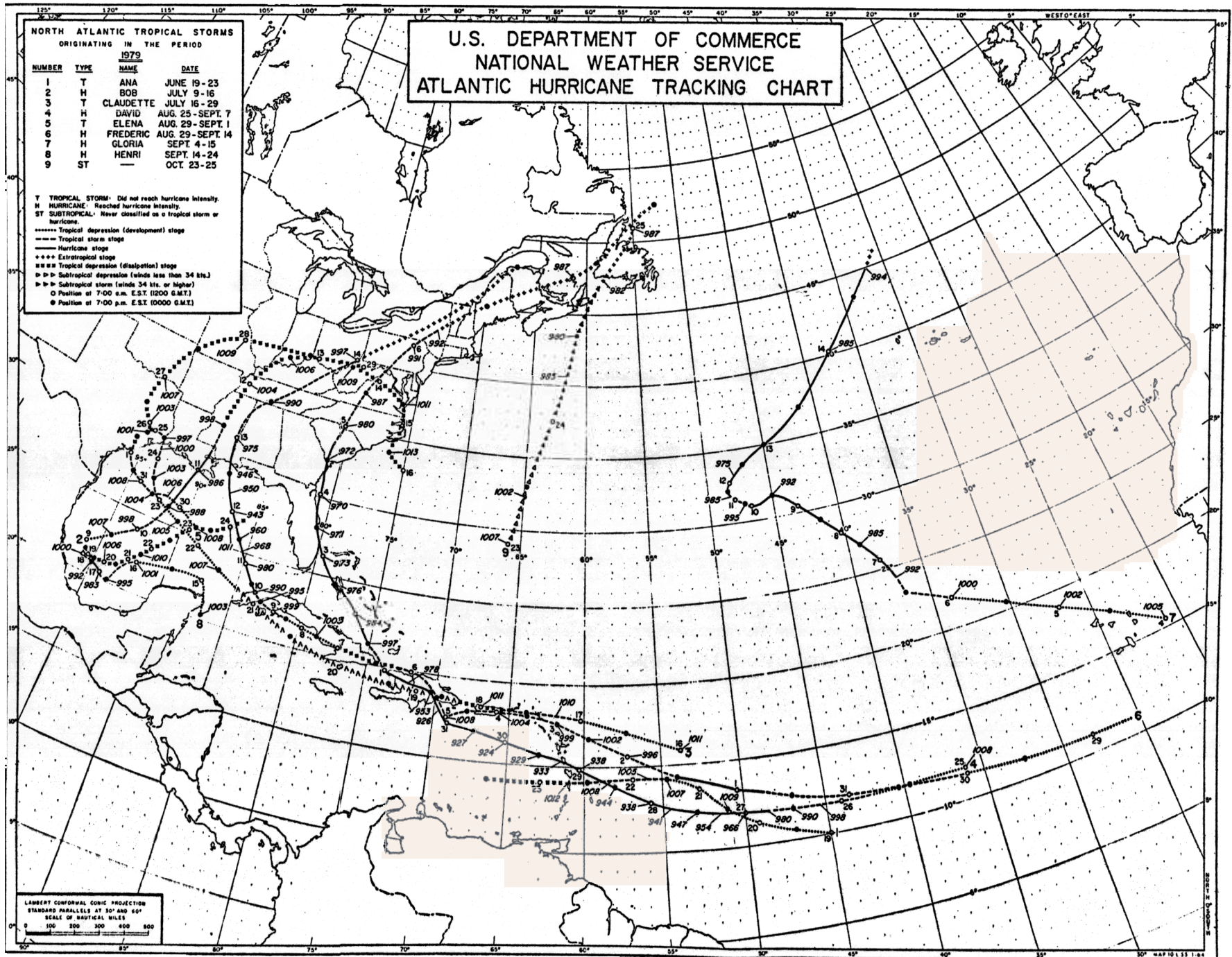
Figure 1. Tracks of 1979 Atlantic tropical and subtropical cyclones.
