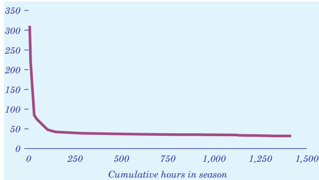
Figure 20. Electricity generation price duration curve for the New England region (1997 mills per kilowatthour)
