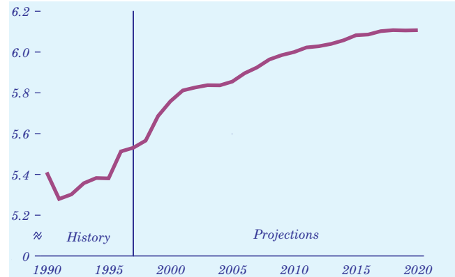
Figure 119. Carbon emissions per capita, 1990-2020 (metric tons per person)
