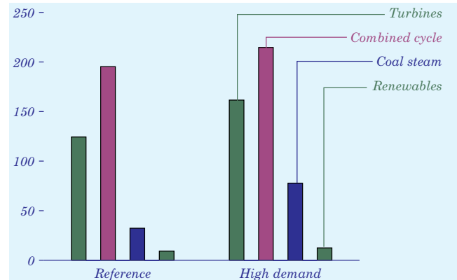
Figure 77. Cumulative new generating capacity by type in two cases, 1997-2020 (gigawatts)
