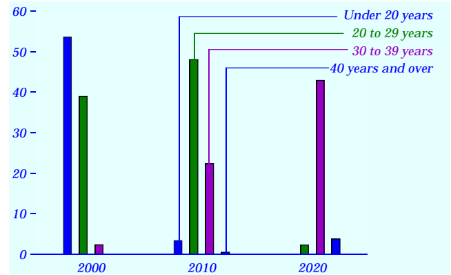
Figure 75. Operable nuclear power capacity by age of plant, 2000, 2010, and 2020 (gigawatts)
