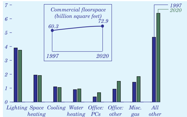
Figure 51. Commercial primary energy consumption by end use, 1997 and 2020 (quadrillion Btu)
