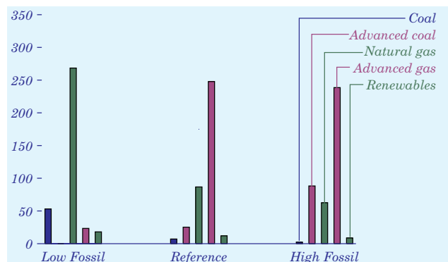
Figure 79. Cumulative new electricity generating capacity by technology type in three cases, 1997-2020 (gigawatts)
