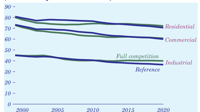
Figure 22. U.S. electricity prices by end-use sector in the reference and full competition cases, 1999-2020 (1997 mills per kilowatthour)
