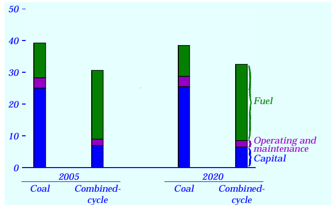
Figure 72. Electricity generation costs, 2005 and 2020 (1997 mills per kilowatthour)
