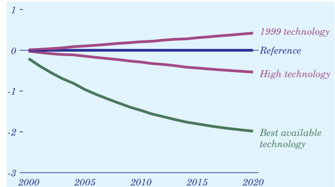
Figure 63. Variation from reference case primary commercial energy use in three alternative cases, 2000-2020 (quadrillion Btu)
