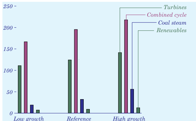
Figure 78. Cumulative new generating capacity by type in three cases, 1997-2020 (gigawatts)
