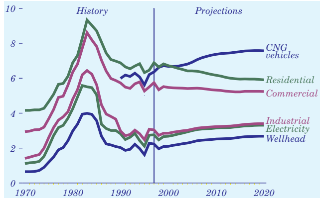
Figure 95. Natural gas end-use prices by sector, 1970-2020 (1997 dollars per thousand cubic feet)
