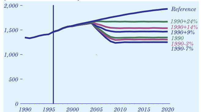
Figure 23. U.S. carbon emissions in seven Kyoto Protocol analysis cases, 1990-2020 (million metric tons)
