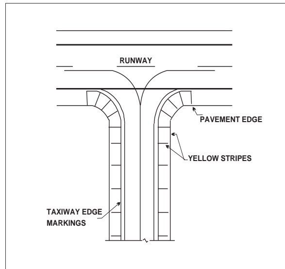
FIG AD 1.1-24 Taxi Shoulder Markings
