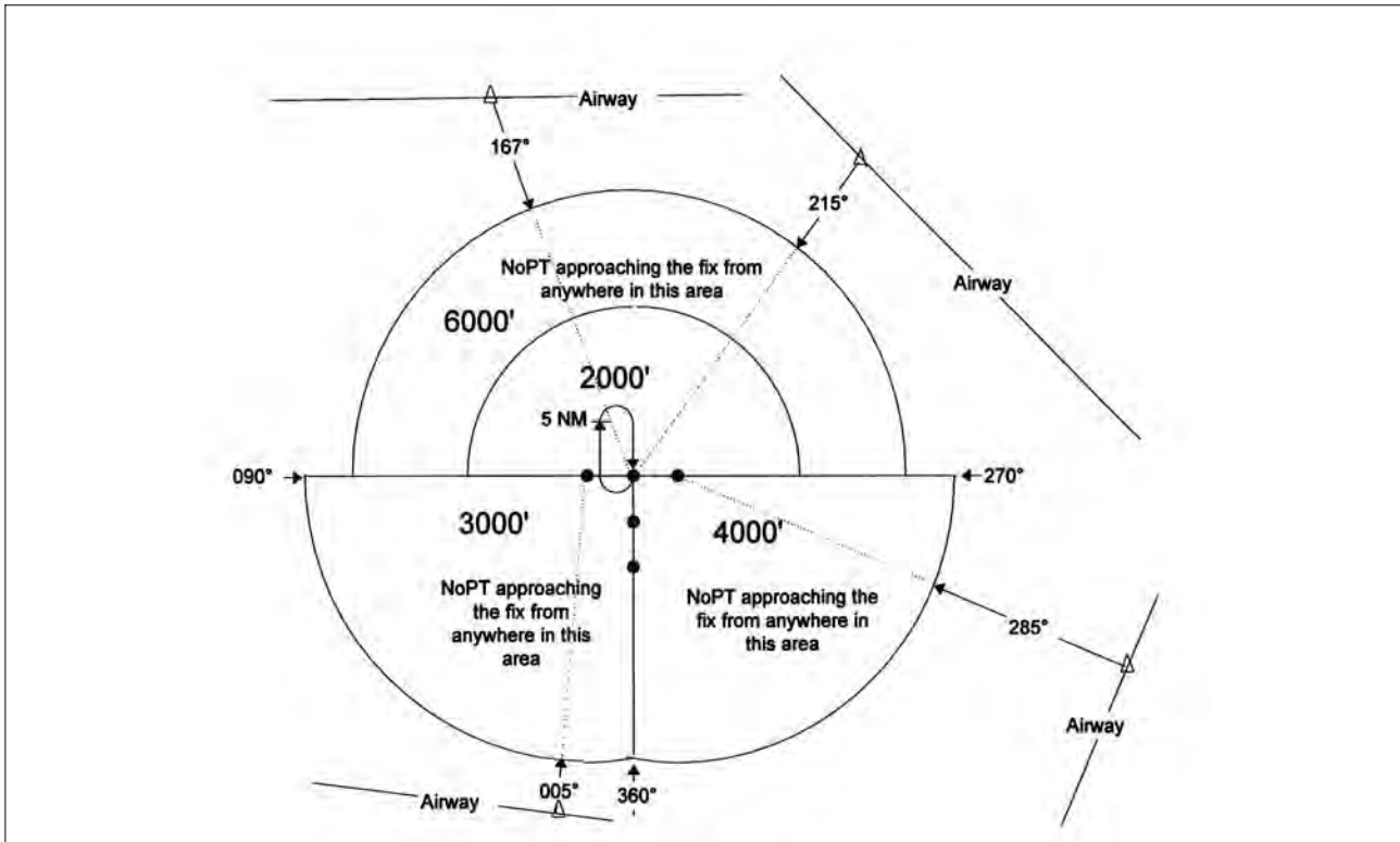
FIG ENR 1.5-26 Examples of a TAA with Feeders from an Airway
