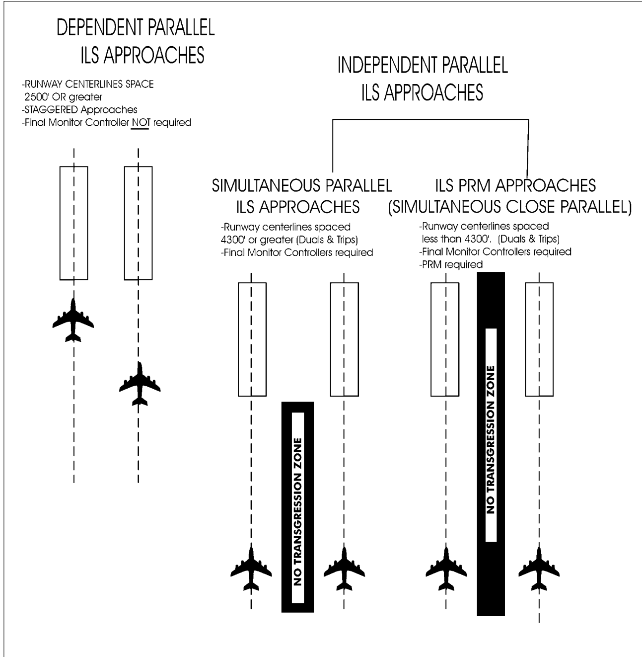
FIG ENR 1.5-28 Parallel ILS Approaches
