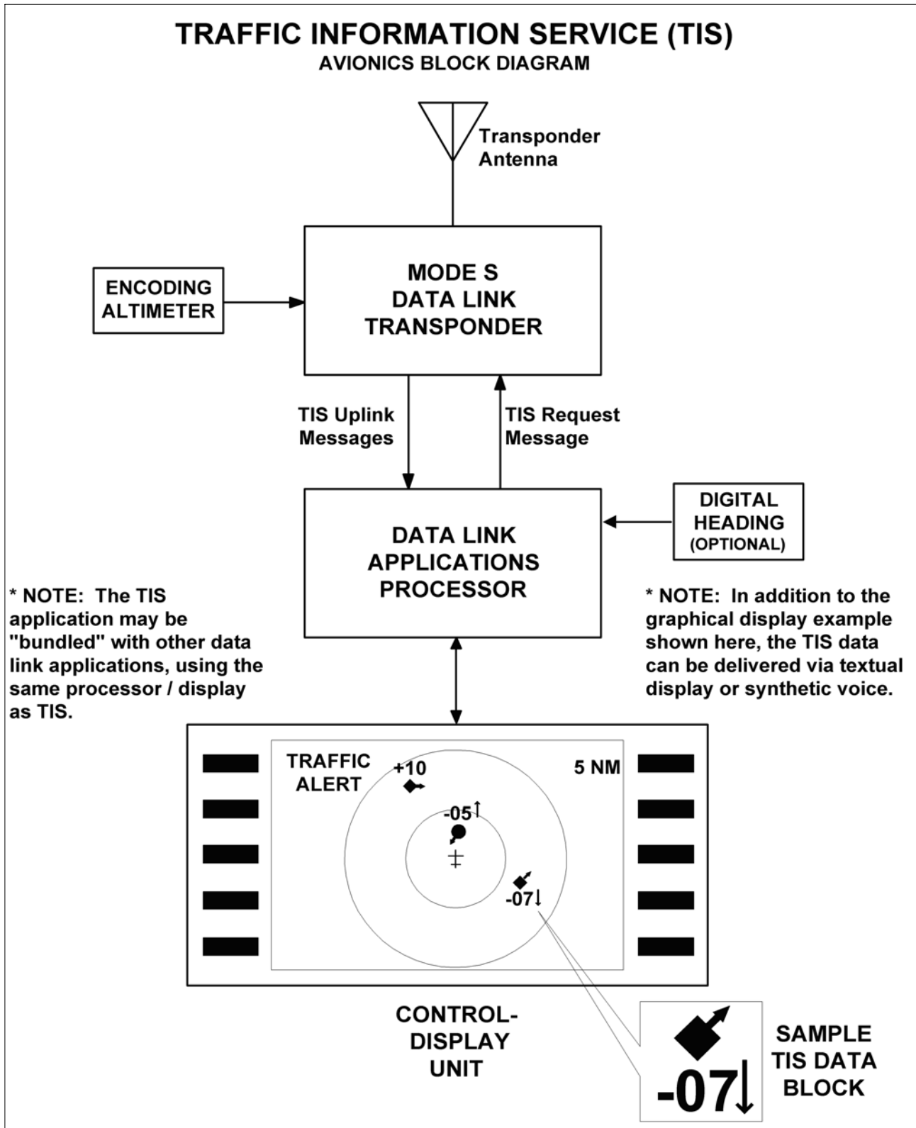
FIG ENR 1.1-31 Traffic Information Service (TIS) Avionics Block Diagram
