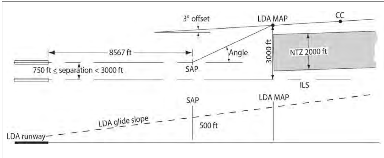
FIG ENR 1.5-32 SOIA Approach Geometry
