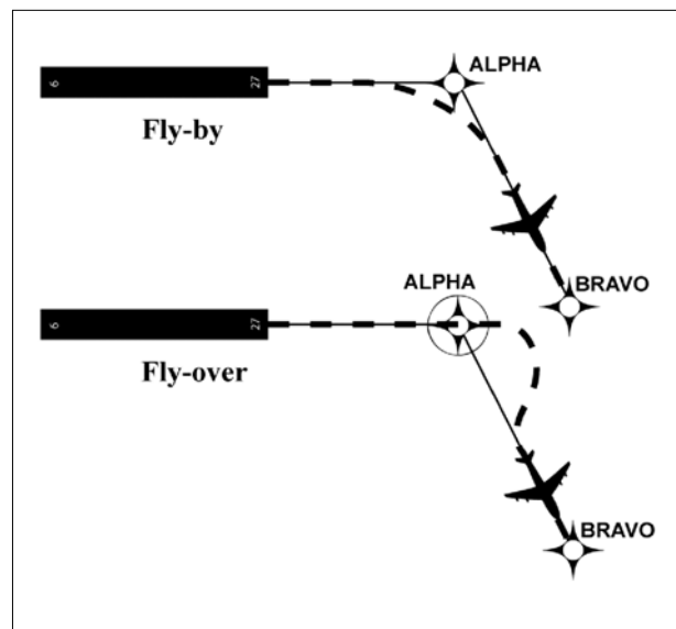
FIG ENR 1.19-1 Fly-by and Fly-over Waypoints
