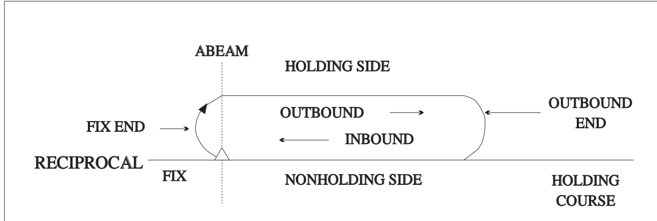
FIG ENR 1.5-2 Holding Pattern Descriptive Terms
