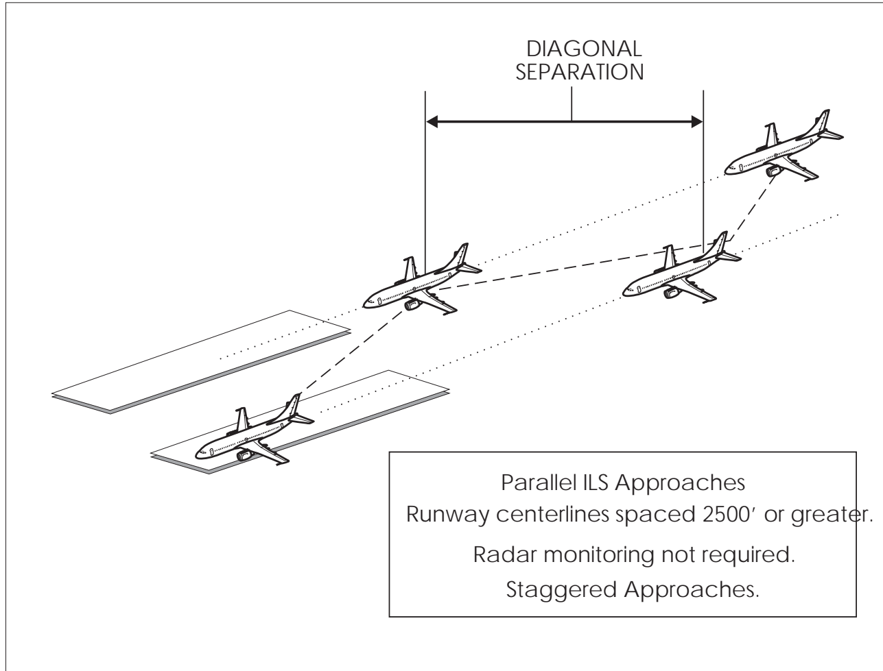
FIG ENR 1.5-29 Staggered ILS Approaches
