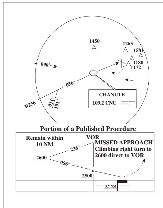
FIG ENR 1.5-35 Missed Approach
