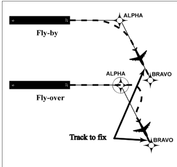
FIG ENR 1.19-2 Track to Fix Leg Type
