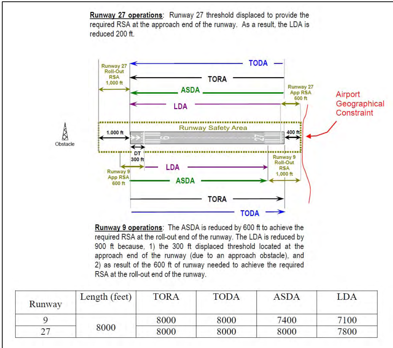
FIG ENR 1.1-5 Effects of a Geographical Constraint on a Runway's Declared Distances
