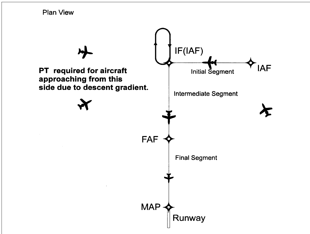
FIG ENR 1.5-17 Modified Basic "T"
