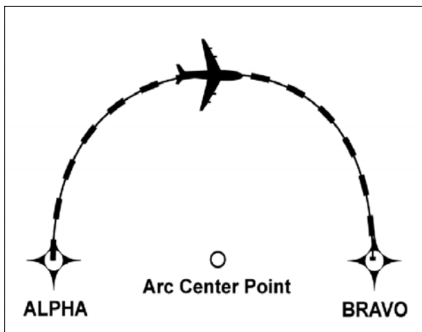
FIG ENR 1.19-5 Radius to Fix Leg Type
