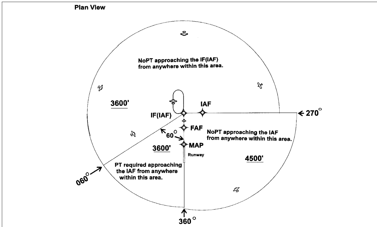
FIG ENR 1.5-25 TAA with Right Base Eliminated
