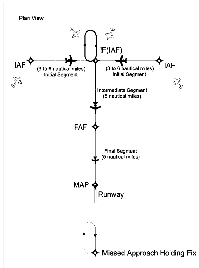
FIG ENR 1.5-15 Basic "T" Design
