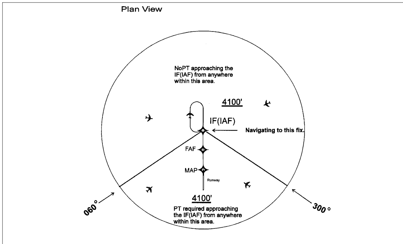
FIG ENR 1.5-24 TAA with Left and Right Base Areas Eliminated
