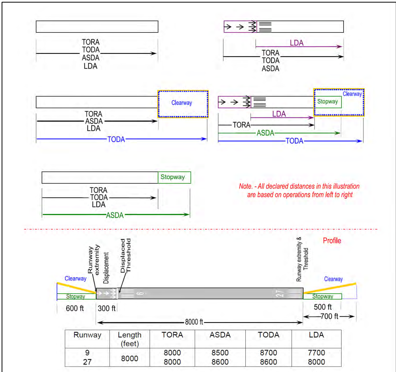
FIG ENR 1.1-4 Declared Distances with Full-Standard Runway Safety Areas, Runway Object Free Areas, and Runway Protection Zones
