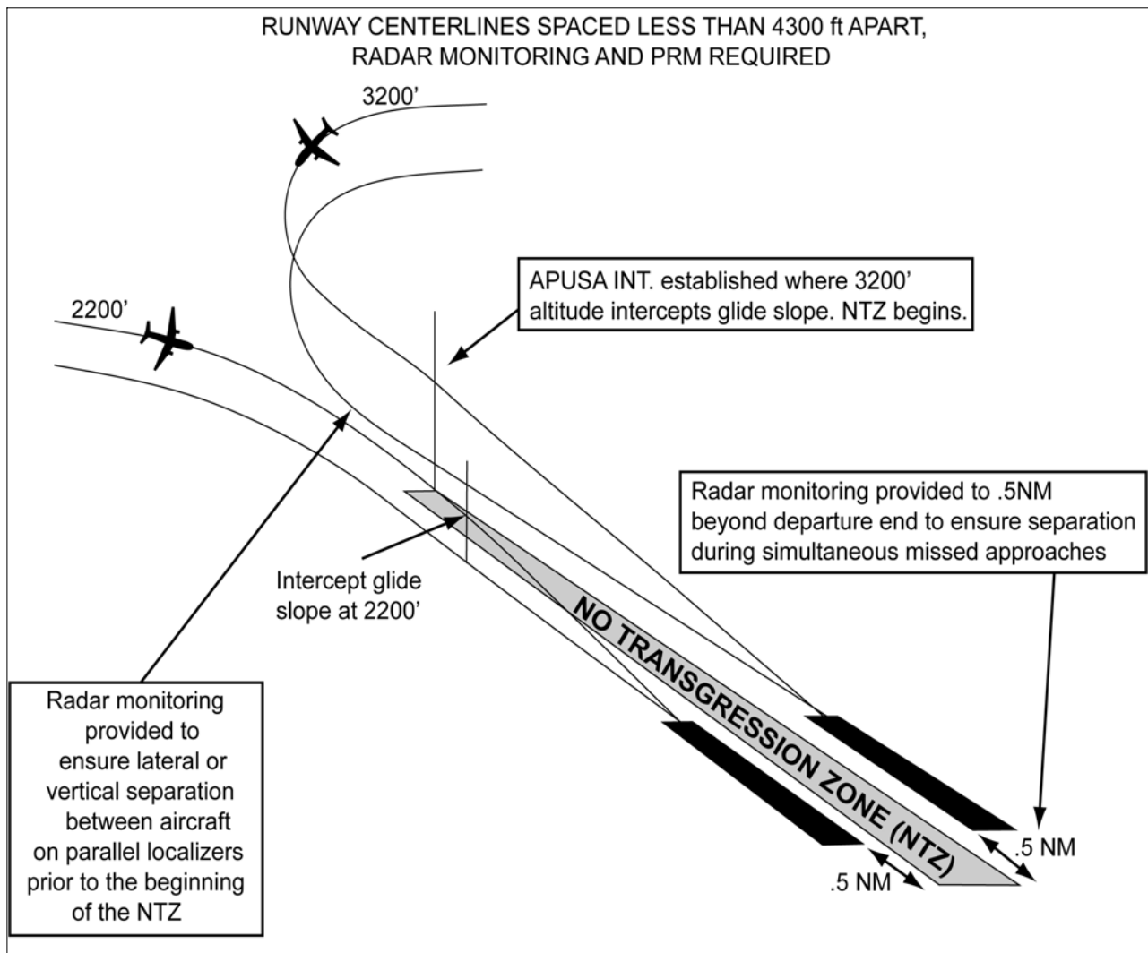
FIG ENR 1.5-31 ILS PRM Approaches (Simultaneous Close Parallel)
