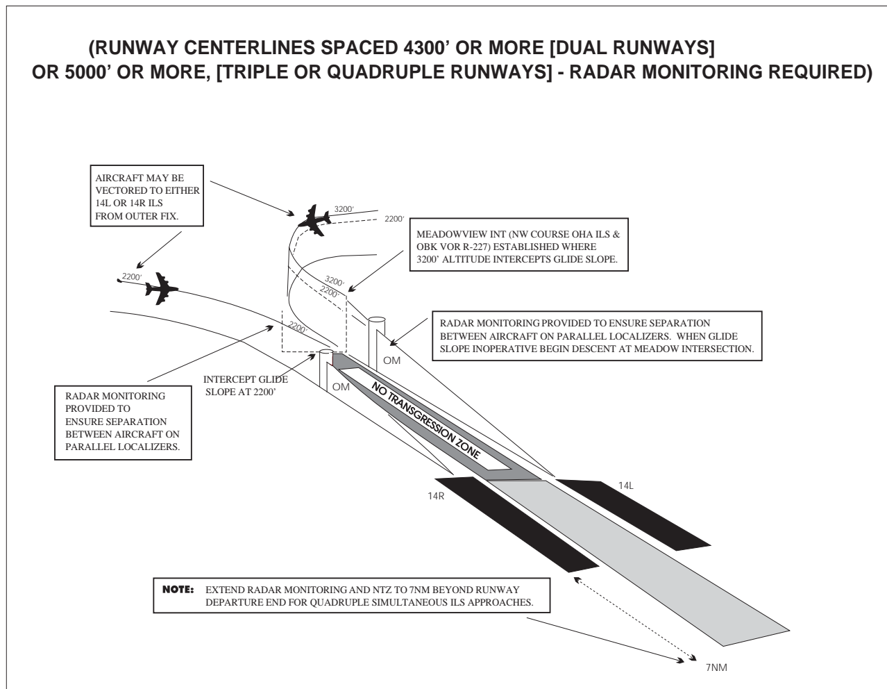
FIG ENR 1.5-30 Simultaneous Parallel ILS Approaches
