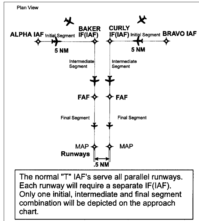
FIG ENR 1.5-18 Modified "T" Approach to Parallel Runways
