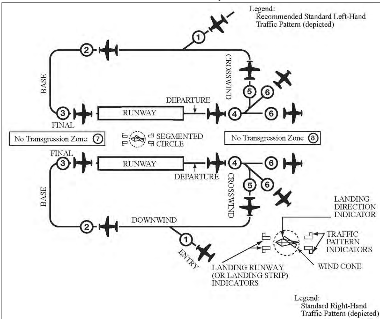
FIG ENR 1.1-3 Traffic Pattern Operations Parallel Runways
