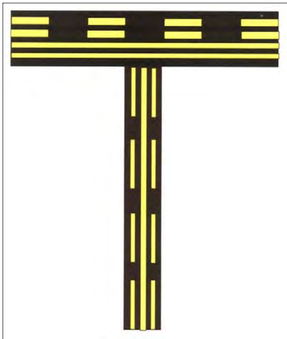
FIG AD 1.1-22 Enhanced Taxiway Centerline
