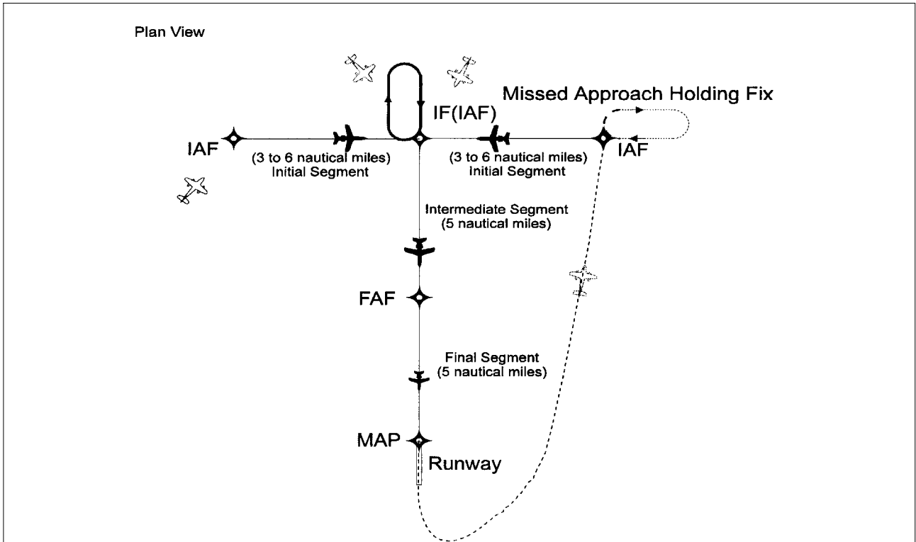
FIG ENR 1.5-16 Basic "T" Design
