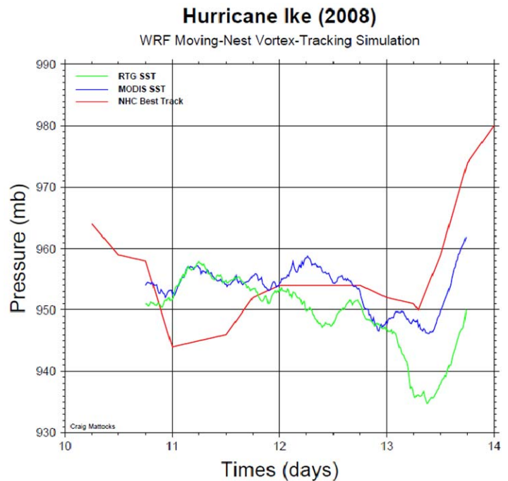
Figure 3. Central pressure (mb) traces from Advanced Hurricane WRF (AHW) simulations of Hurricane Ike (2008) using 50 km horizontal resolution real-time global SST analyses (green) and 1 km horizontal resolution NASA-Marshall SPoRT MODIS SST analyses (blue). The NHC best track central pressure trace is shown in red.
