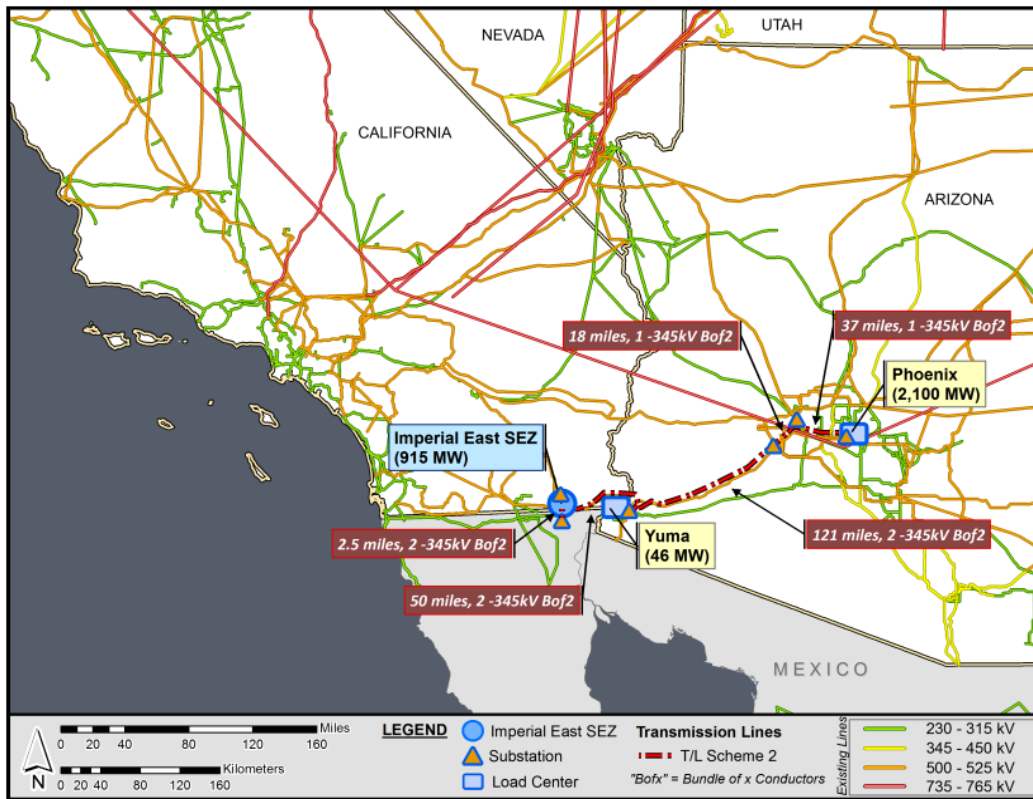
1 2 FIGURE 9.1.23.1-3 Transmission Scheme 2 for the Proposed Imperial East SEZ 3 (Source for background map: Platts 2011)
