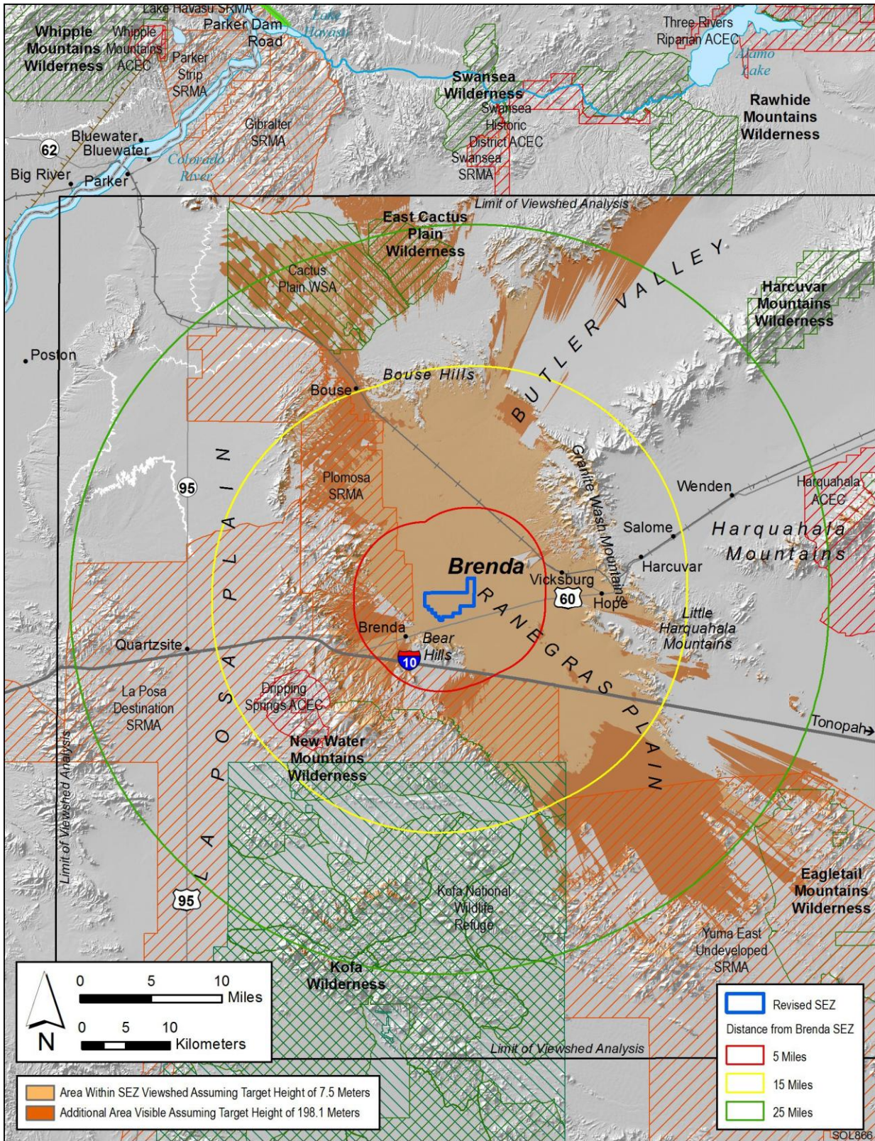
2 FIGURE 8.1.14.2-2 Overlay of Selected Sensitive Visual Resource Areas onto Combined 650-ft 3 (198.1-m) and 24.6-ft (7.5-m) Viewsheds for the Proposed Brenda SEZ as Revised
