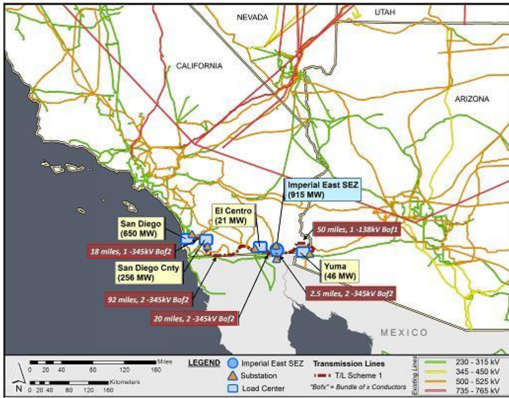
2 FIGURE 9.1.23.1-2 Transmission Scheme 1 for the Proposed Imperial East SEZ 3 (Source for background map: Platts 2011)
