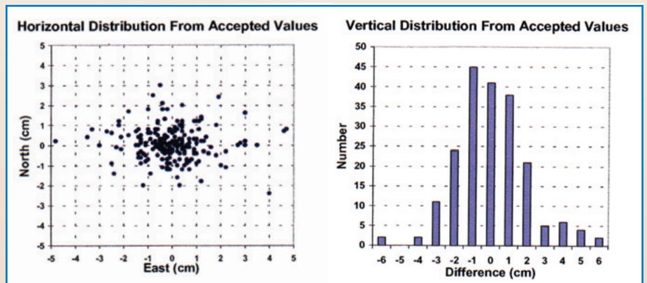
Figure 2 The horizontal and vertical distributions of OPUS solution differences from accepted ITRF values are shown for over 200 CORS stations using only two hours of data, the minimum required by OPUS. The standard deviations of these results are 0.8, 1.4, and 1.9 cm for the north, east and up dimensions respectively. All mean differences were less than 1 mm.
