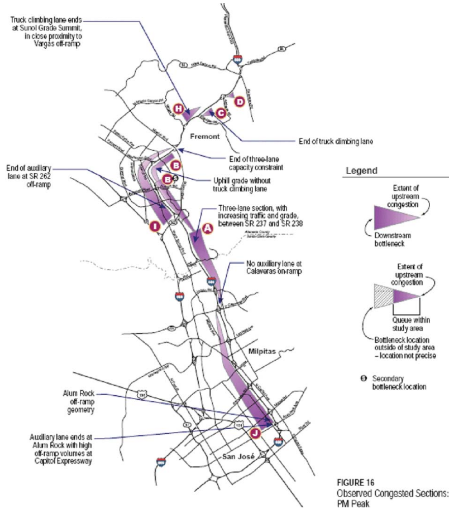
Figure 11. Bottleneck Locations
