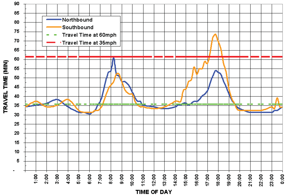
Figure 6. Mobility-Travel Time
