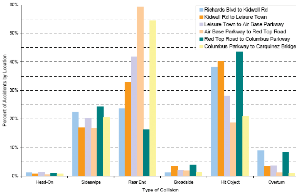
Figure 14. Safety-Accident Rates
