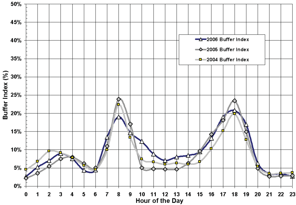
Figure 12. Reliability-Buffer Index
