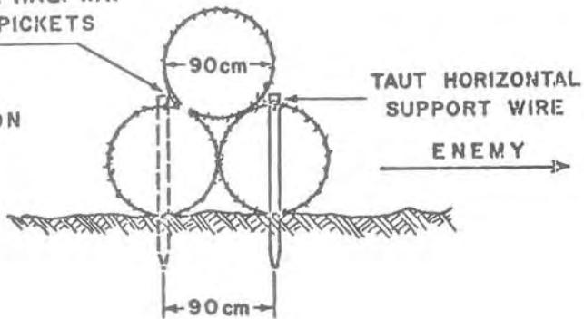
Figure 3-1. Triple Standard Concertina Fence.
