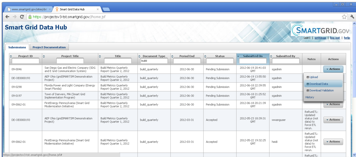
Figure 5: Selecting Download Data action via the Action button.
