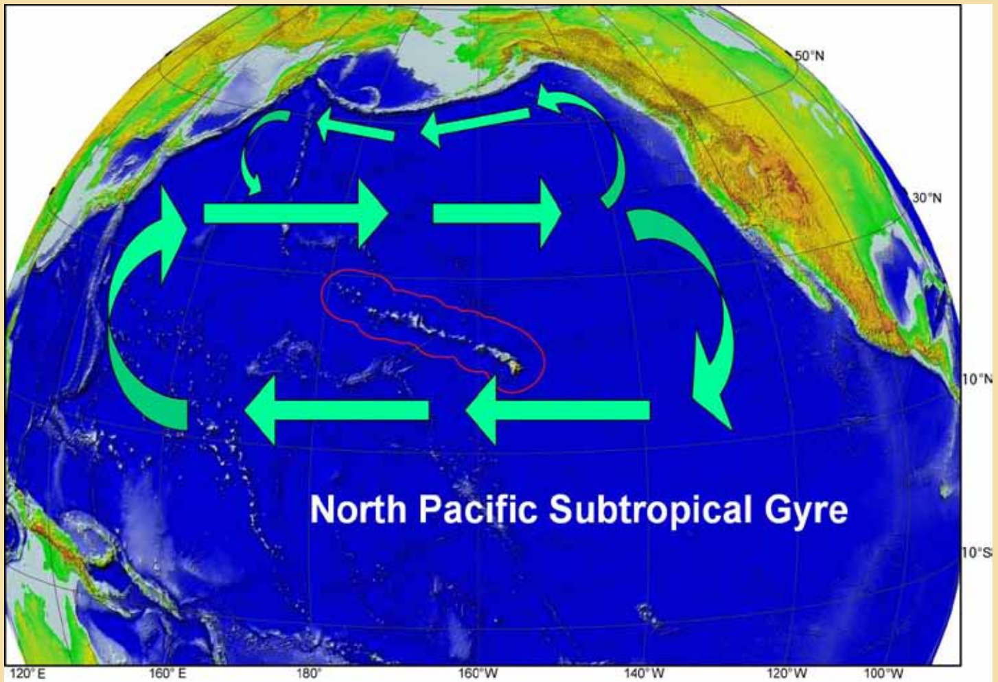
Current diagram of the Pacific Ocean illustrating the North Pacific Subtropical Gyre.
