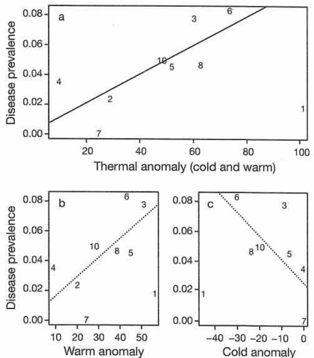
Fig. 5. Regional mean coral disease prevalence by proportion of corals with disease and temperature indices showing (line) significant linear regression fit. Numbers correspond to regions. See Table 1 for region descriptions. (a) Disease prevalence regressed against accumulated thermal stress, which was determined by adding SST3, the summation of sea surface temperatures over the mean plus 1°C, with SST4, the summation of sea surface temperatures under the mean minus 1°C (adjusted R^2 = 0.5478 , p = 0.0217 ). (b) Disease prevalence against warm anomaly (adjusted R^2 = 0.38 , p = 0.0596 ). (c) Disease prevalence against cold anomaly (adjusted R^2 = 0.32 , p = 0.0805 ). Data corresponding to Panama were not available to be included in this analysis. 1: Bermuda, 2: Cayman Islands, 3: Curacao, 4: Great Barrier Reef, 5: Grenada, 6: Mexican Yucatan, 7: Northwestern Hawaiian Islands, 8: Philippines, 9: Panama, 10: Puerto Rico
