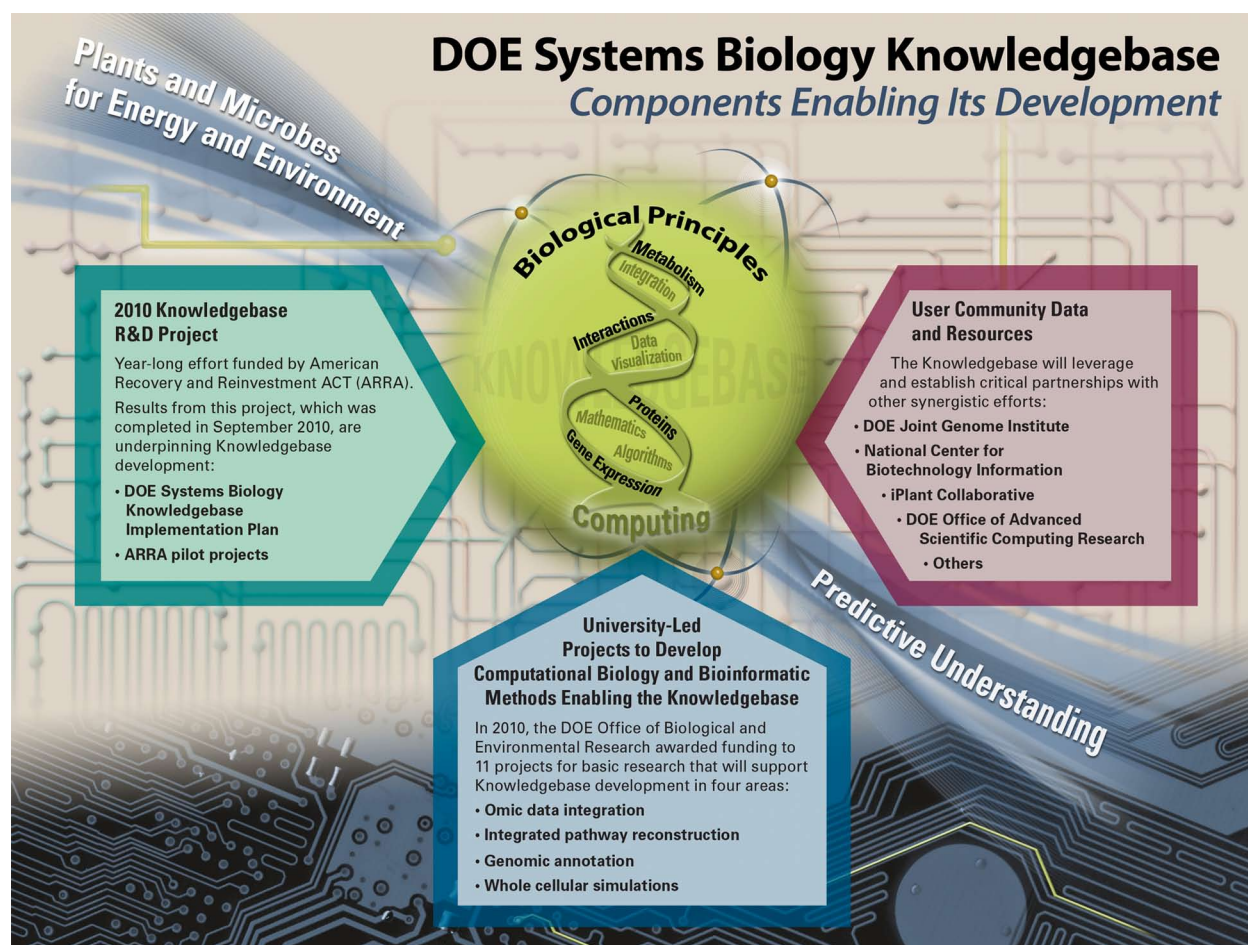
Fig. 2. DOE Systems Biology Knowledgebase.
