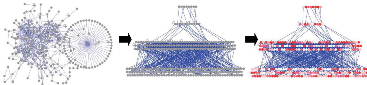
Fig. 6. Schematic Representing Effects of Rewiring a Transcriptional Regulatory Network in a Hierarchical Context. Related to the second aim, researchers performed a topological network analysis in correlation with genome-wide phenotypic data. (1) The transcriptional regulatory network is first arranged into a hierarchy, with the regulatory edges pointing only downward. To mimic the commonplace government and corporate hierarchy, no regulator controls any gene above it in the hierarchy. (2) Phenotypic effects of tampering with various nodes and edges (e.g., their removal or additions) on cell growth and survival are overlaid onto the hierarchy. Different genes have different effects on cell growth. (3) Node color (scaling from white to red) indicates the effect of tinkering on cell growth and survival. Tampering with white nodes has a minimal effect (cell grows normally), whereas red nodes are the genes that, upon deletion, affect cell growth adversely (cell grows at a slower rate or dies). Researchers find that tampering with upper-level nodes affects cell growth more adversely. [From Bhardwaj, N., et al. 2010. "Rewiring of Transcriptional Regulatory Networks: Hierarchy, Rather Than Connectivity, Better Reflects the Importance of Regulators," Science Signaling 3 (146), ra79. Reprinted with permission from AAAS.]
