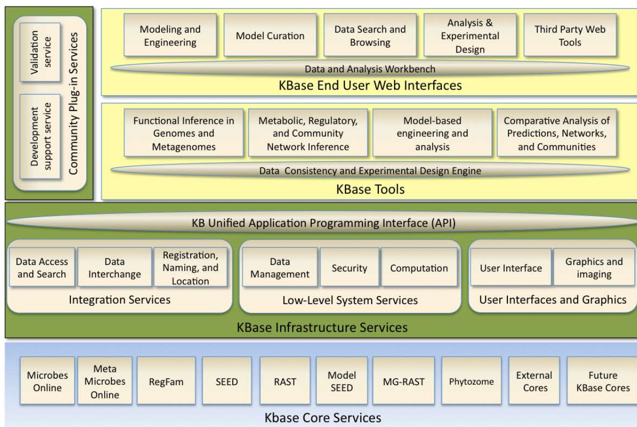
Fig. 3. Kbase Architecture.
