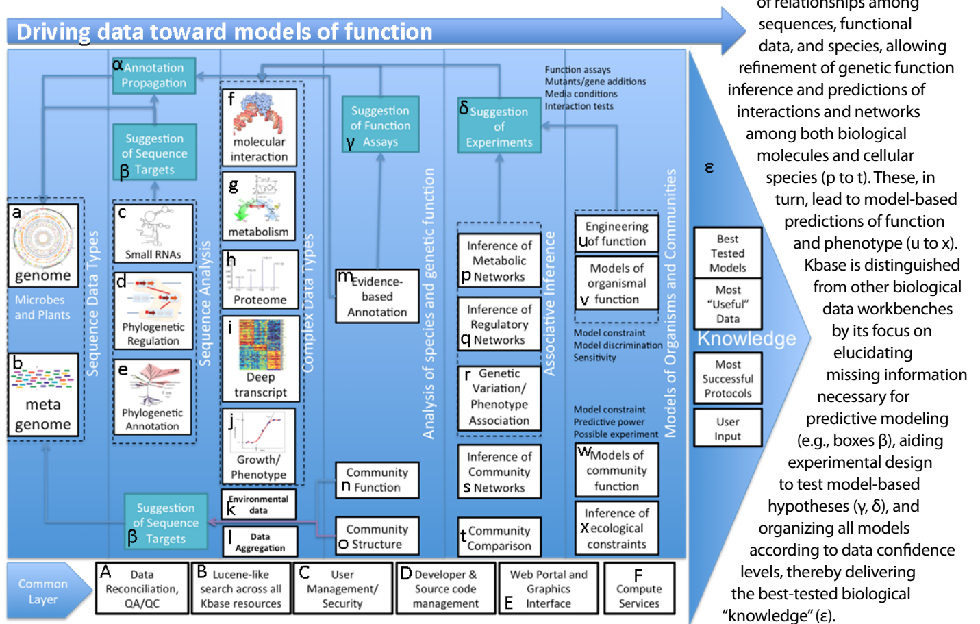
Fig. 4. Toward Predictive Capability. Kbase seeks to drive data toward dynamic, testable models of gene and network function and dynamic behavior in an environmental context. The progression is shown from left to right in the middle: sequence data is annotated first using comparative methods (a to e) and then increasingly with functional data (f to o). The annotations and data lead to inferences
