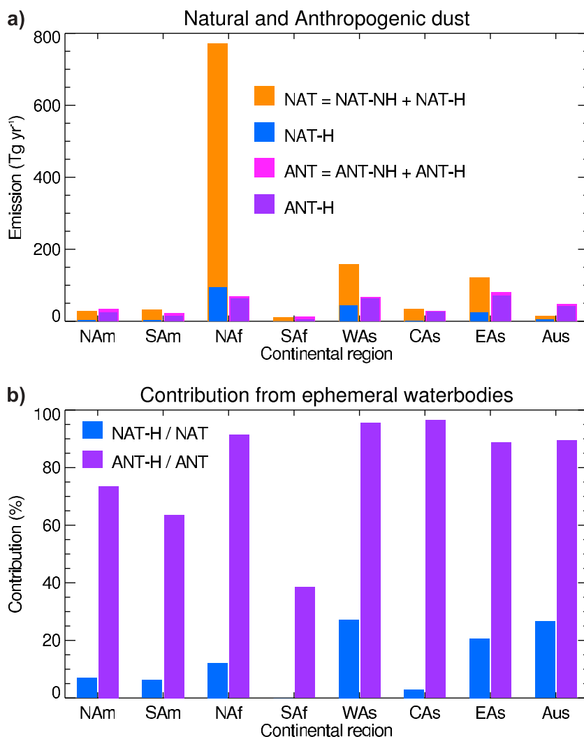
Figure 17. (a) Annual mean emission ( \text{Tg yr}^{-1} ) over North America (NA m ), South America (SA m ), North Africa (NA f ), South Africa (SA f ), West Asia-Middle East (WAs), Central Asia (CAs), East Asia (EAs), and Australia (Aus) from natural (NAT-H + NAT-NH), anthropogenic (ANT-H + ANT-NH), and natural (NAT-H) and anthropogenic (ANT-H) sources with more than 10% ephemeral water bodies per grid cell. (b) The percentage contribution of ephemeral water bodies to natural and anthropogenic emissions for each continental region.
