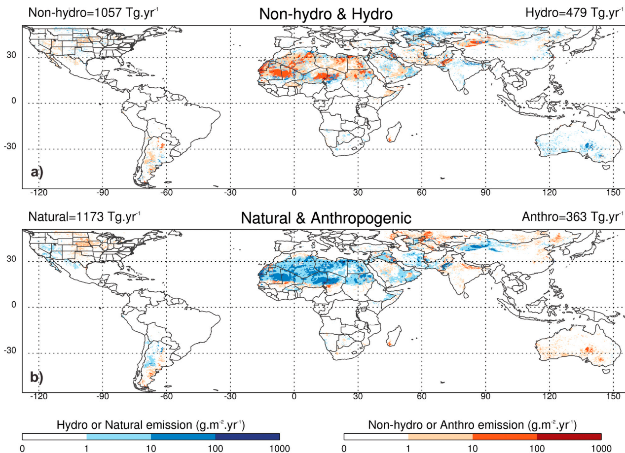
Figure 16. Annual mean dust emission (a) from ephemeral water bodies and (b) from land use. The M-DB2 emissions are colored in blue for hydrologic and natural sources and in red for nonhydrologic and anthropogenic sources.
