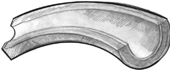
Cross section of a healthy blood vessel
