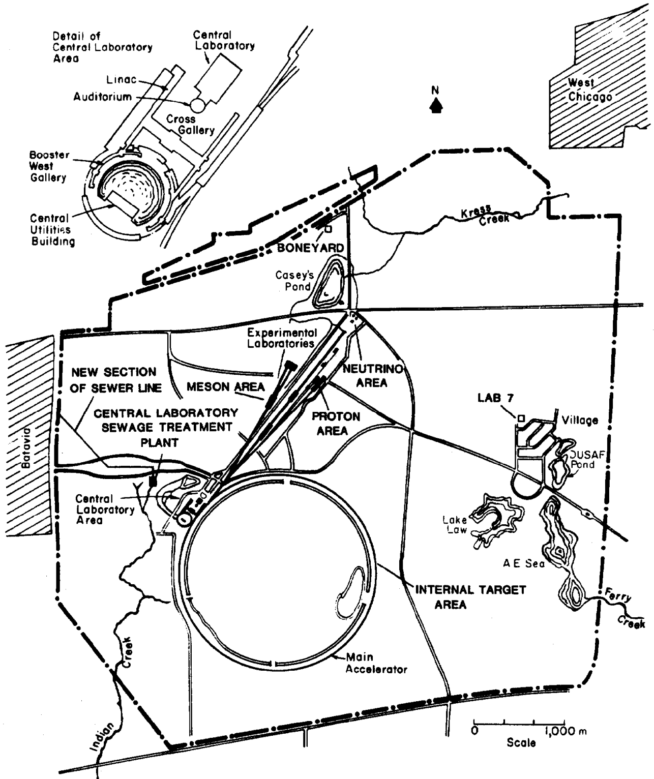
Figure 1. - Fermilab Site
