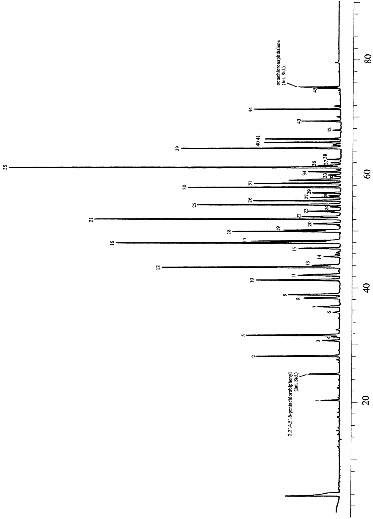
Figure 1. Gas chromatogram from the analysis of SRM 3086 (Aroclor 1260 in Methanol). The 45 peaks used for quantification of the Aroclor mass in solution are shown. (Int. Std.) = internal standard
