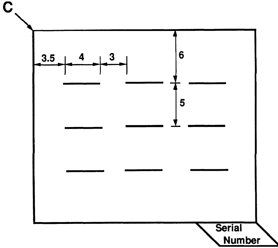
Figure 2. Measurement Positions for SRM 2071. Positions of traces in mm with respect to the upper left corner, C, of the roughness area.
