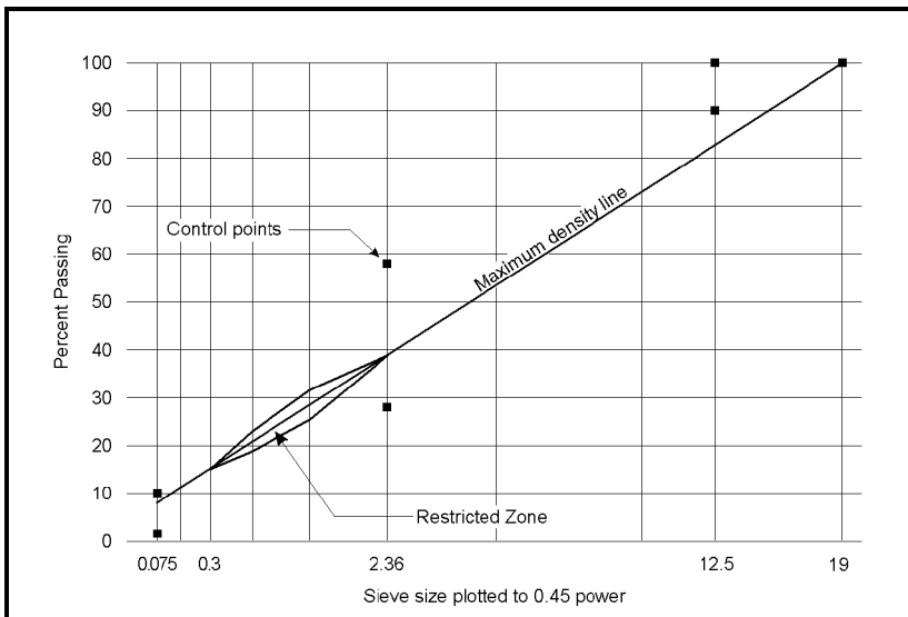
Figure 703-1 Gradation Chart for 12.5-mm Nominal Maximum Size Aggregate
