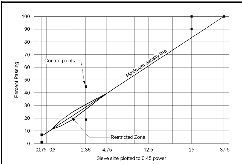
Figure 703-3 Gradation Chart for 25-mm Nominal Maximum Size Aggregate
