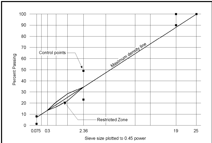
Figure 703-2 Gradation Chart for 19-mm Nominal Maximum Size Aggregate
