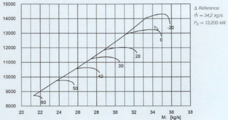
Measured performance map of integrally geared CO 2 compressor
