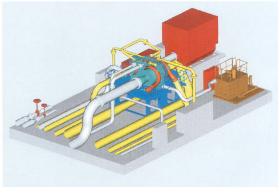
3-D computer model showing compressor, drive motor and lube oil system with interconnecting pipe arrangement to remote intercooler
