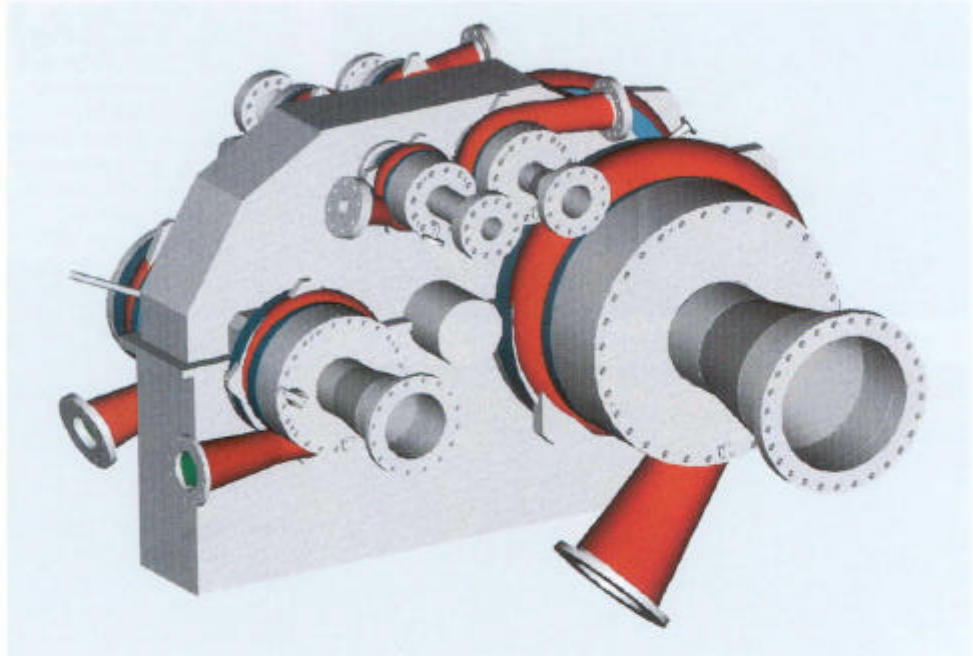
3-D computer model showing arrangement of volutes
