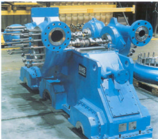
New gear concept with two horizontal shafts ensures excellent maintainability
