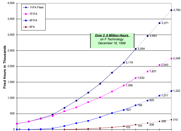
Figure 7. F/FA machines have accumulated over 2.6 million operating hours in all operating modes and now have an accumulation rate of over 100,000 hours per month
