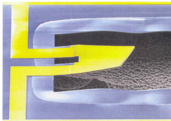
Science 's Breakthrough of the Year goes to the first mechanical, vibrating device, which is as long as a hair is wide. The device is the first to reach the quantum ground state, a feat achieved by physicists at the University of
