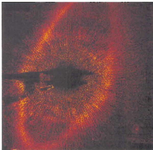
First optical images of an extrasolar planet orbiting a star 25 light years from Earth. Fomalhaut b is 100 million times fainter than the star and sits just inside a vast dust belt circling the star. This image is associated with research by Dr. Paul Kalas and colleagues that appeared in the 13 November 2008 issue of Science Express .
