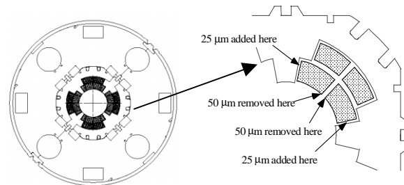
Fig. 2. Left: cold mass cross-section. The coil bore diameter is 70 mm. Right: illustration of the coil shimming which was done to correct b6.
