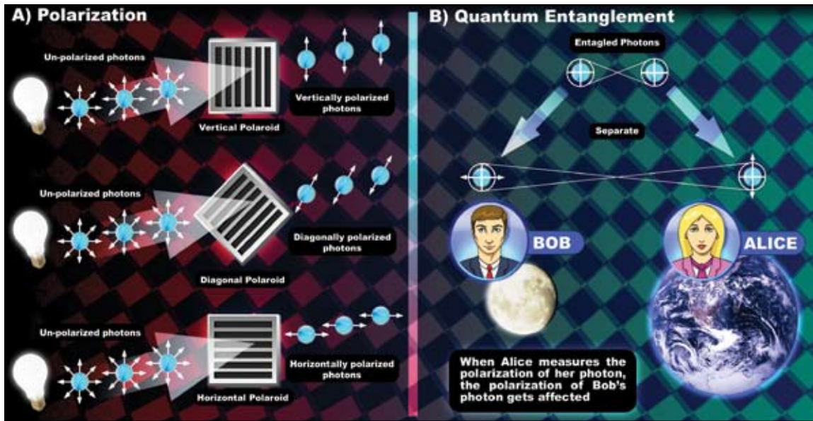
When photons travel, they vibrate, and the direction in which they vibrate is called “polarization.” In figure A, photons can be forced to vibrate in certain directions (vertically, diagonally, or horizontally) by passing them through a filter known as a Polaroid. Figure B portrays quantum entanglement, a concept of fundamental importance for quantum communication. Two photons have become entangled. They then no longer have individual quantum states; they are interrelated.
