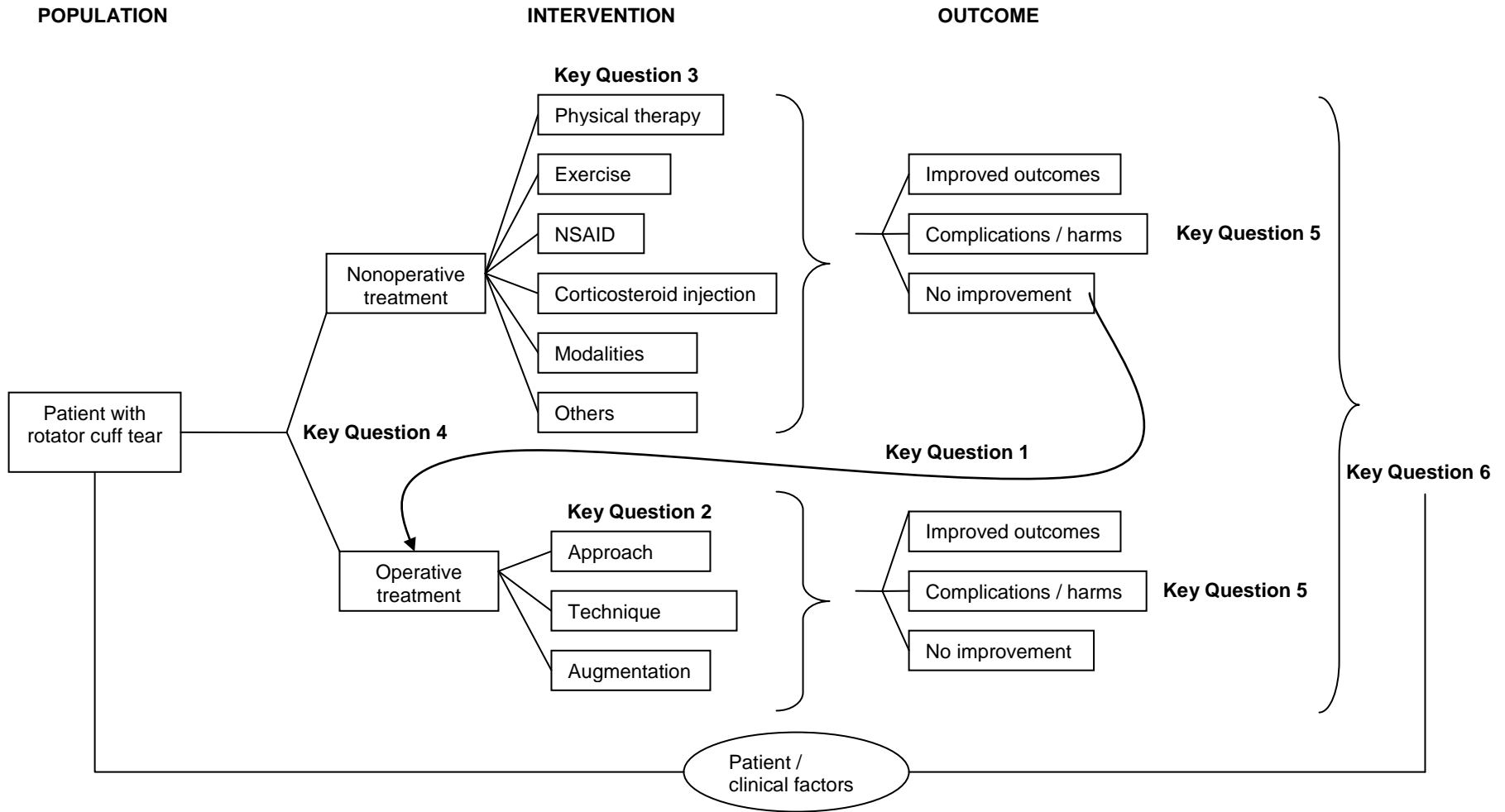
Figure 1. Analytic framework
