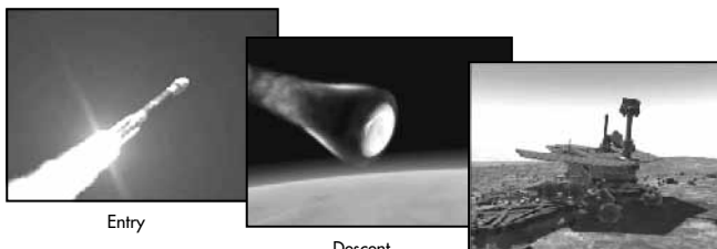
Images courtesy of NASA/JPL
