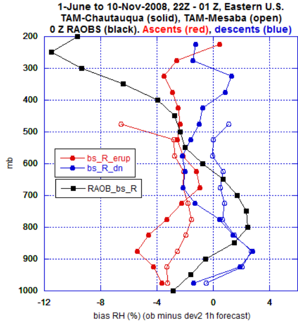
Fig. 22. Relative humidity “bias” (observations minus dev2 1-h forecasts) for TAMDAR-Chautauqua (solid circles), TAMDAR-Mesaba (open circles) and 0 UTC RAOBs (black squares). Ascents are shown in red; descents in blue.
