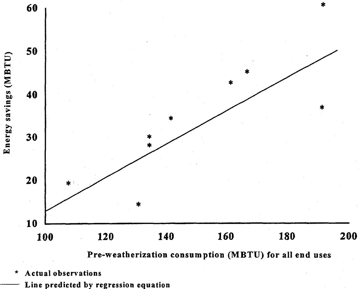
Figure 2. Plot of energy savings by pre-weatherization consumption for gas-heated structures.
