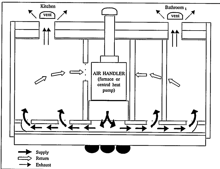
Mobile Home Heating System Distribution System
