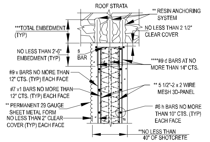
TYPICAL SECTION C-C NOT TO SCALE
