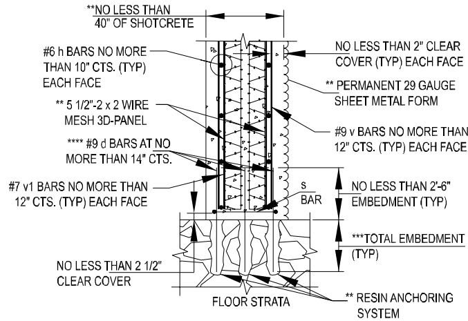
TYPICAL SECTION A-A NOT TO SCALE
