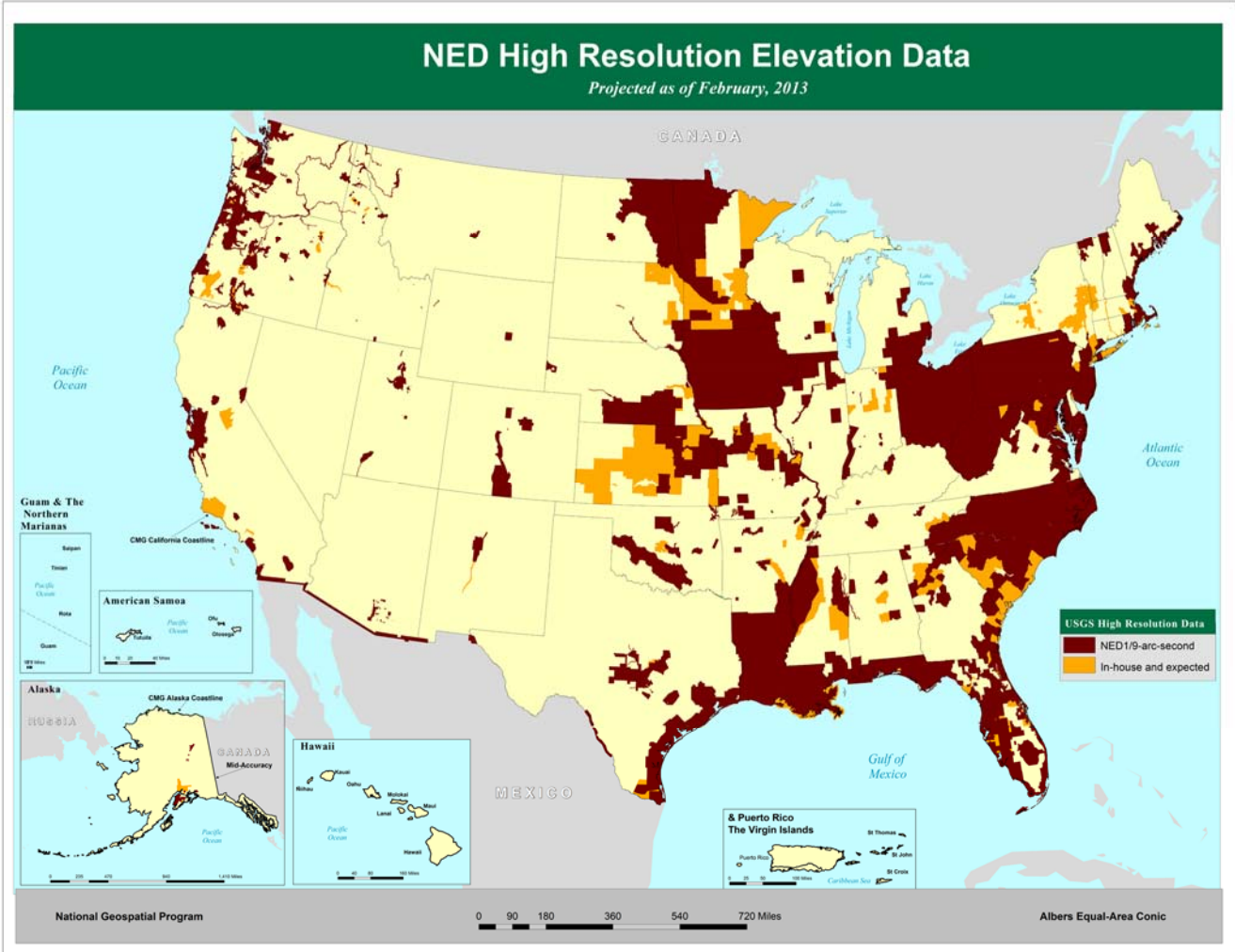
Figure 6. Available and anticipated high-resolution data – February, 2013 release.
