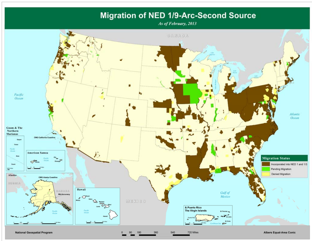
Figure 9. Migration status of NED 1/9 to other NED layers—February, 2013 release.
