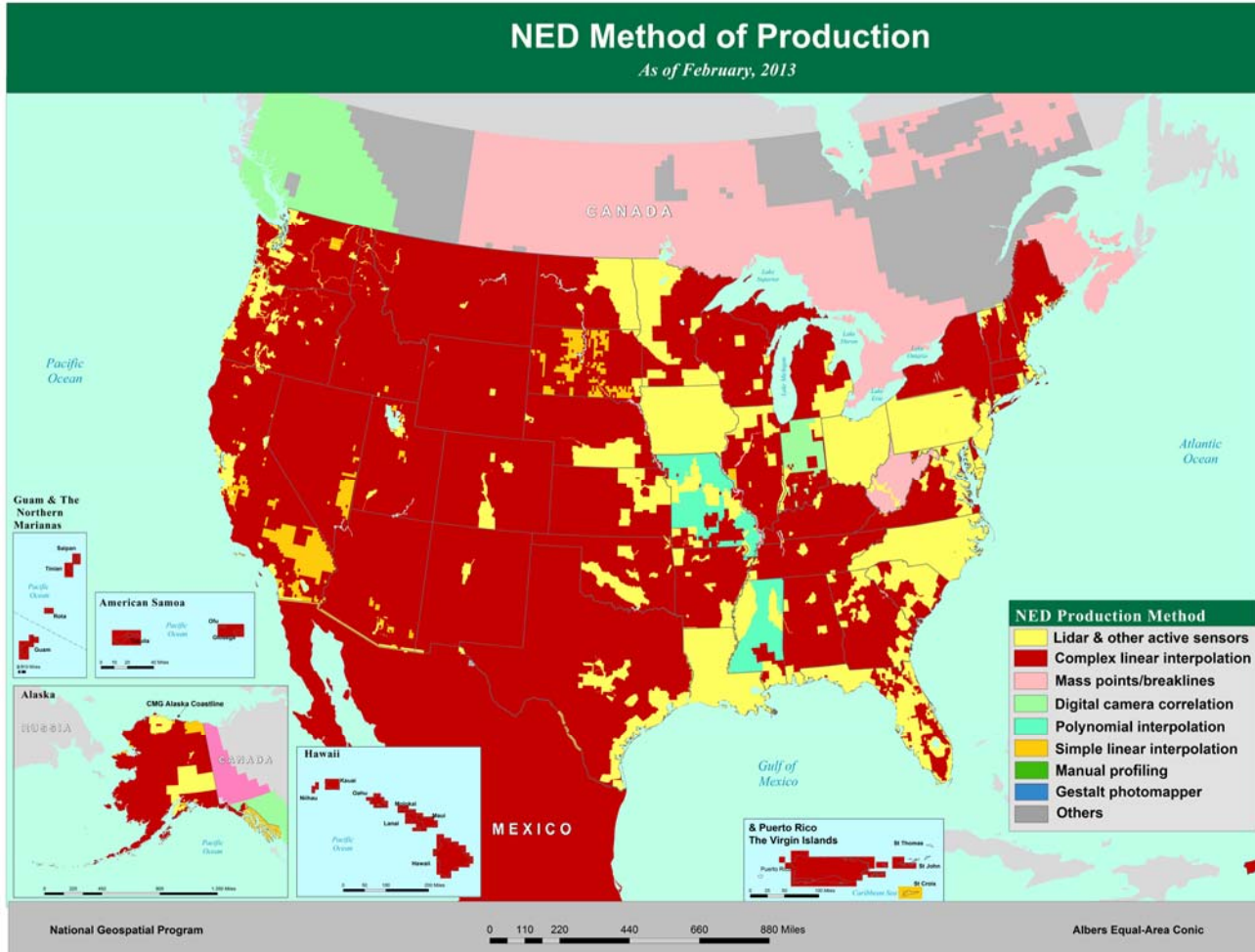
Figure 12. NED source data by production method – February, 2013 release.
