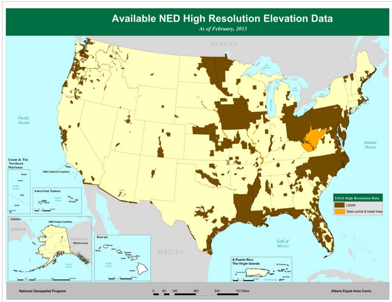
Figure 5. Available 1/9-arc-second data from all sources – February, 2013 release.
