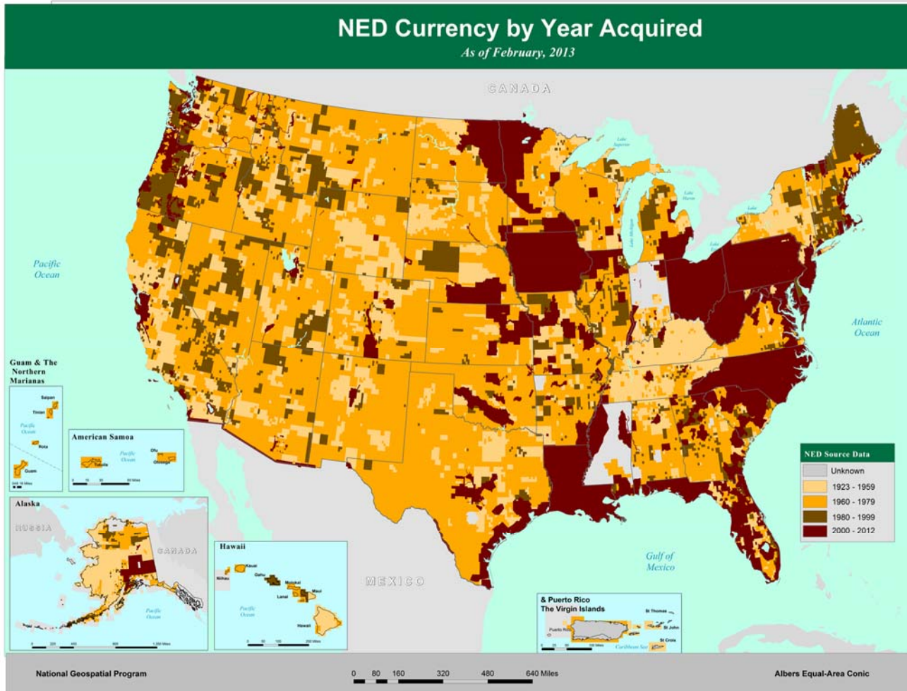
Figure 11. Currency of the NED shown by acquisition year – February, 2013.
