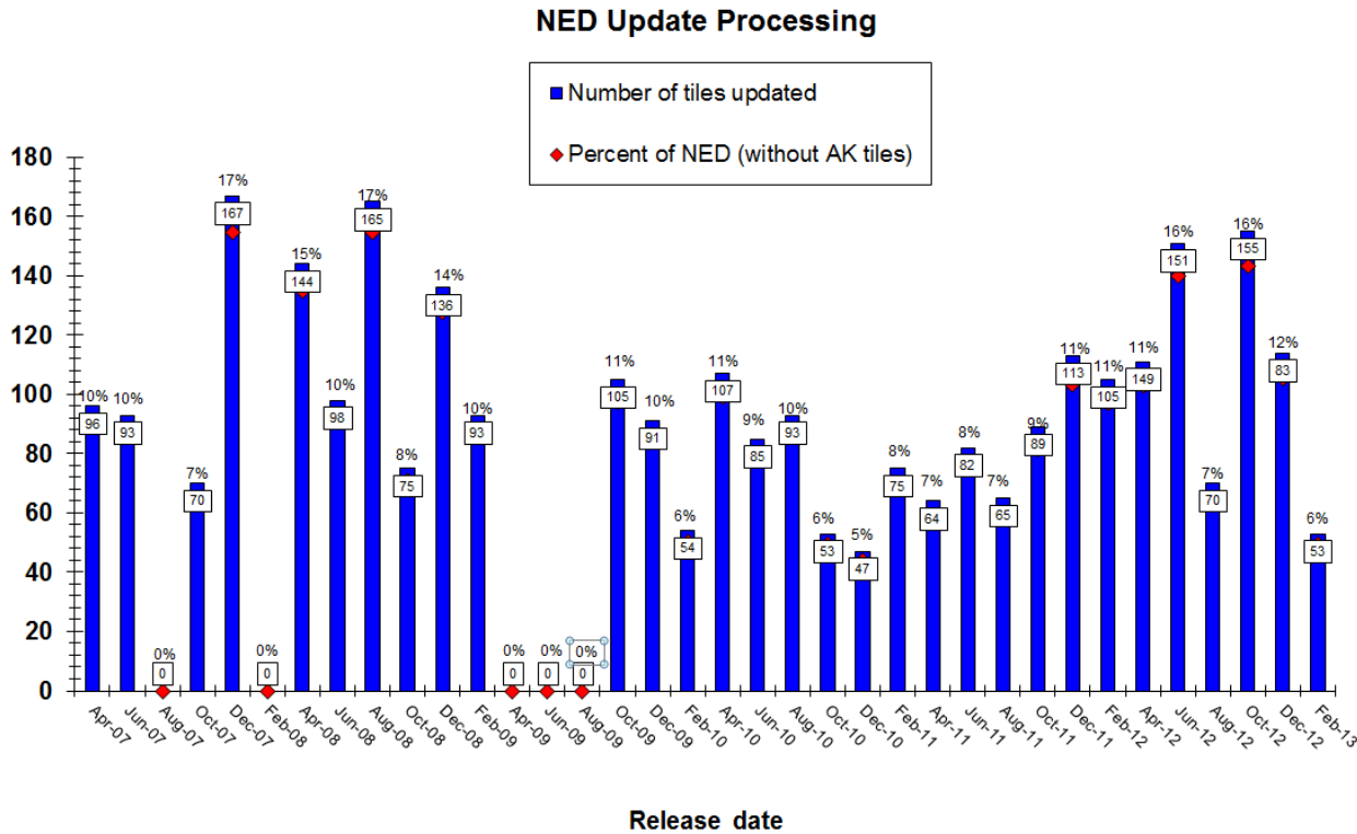
Figure 14. Number and percentage of NED tiles processed by release date.
