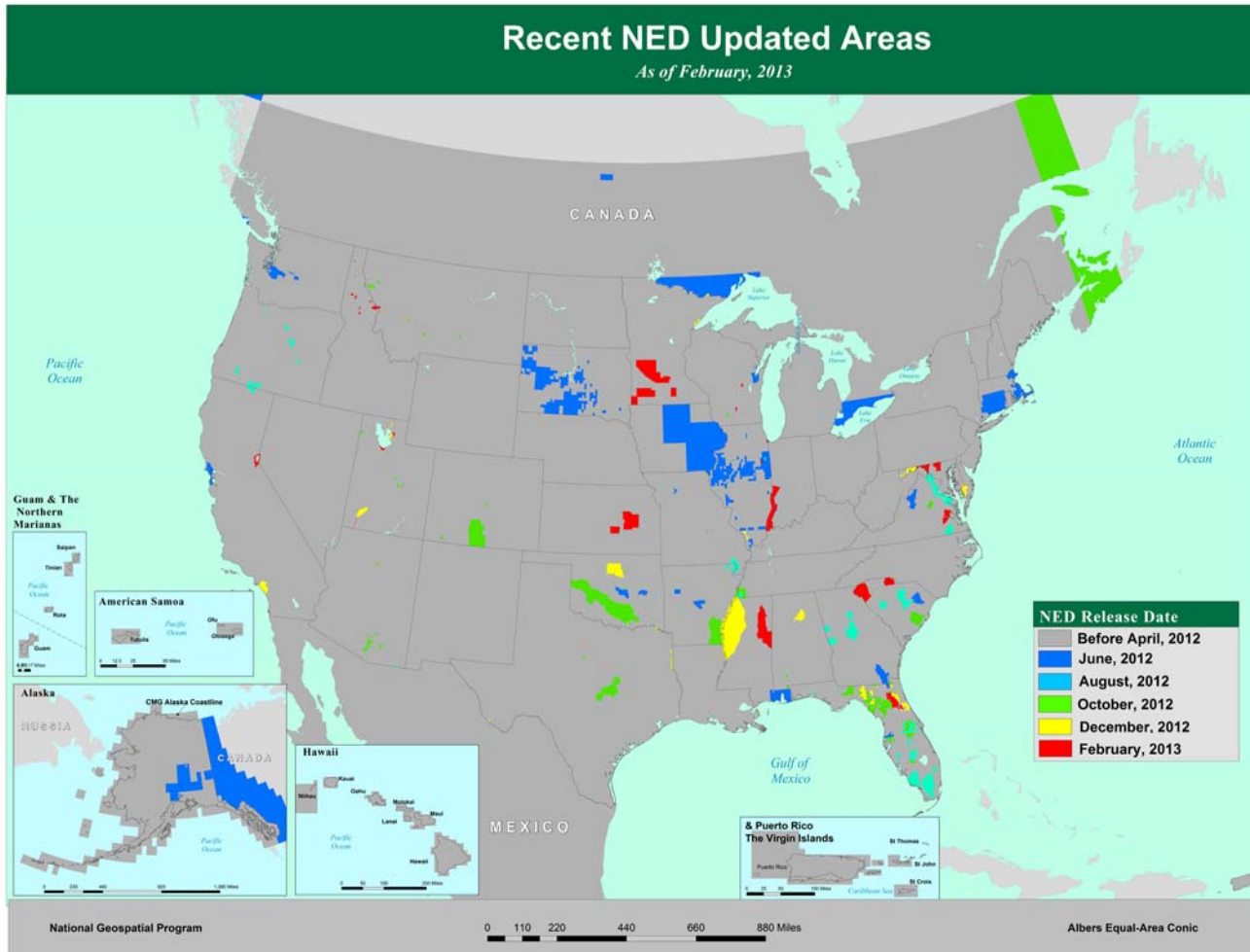
Figure 3. NED updated areas by release date -- February, 2013 release.
