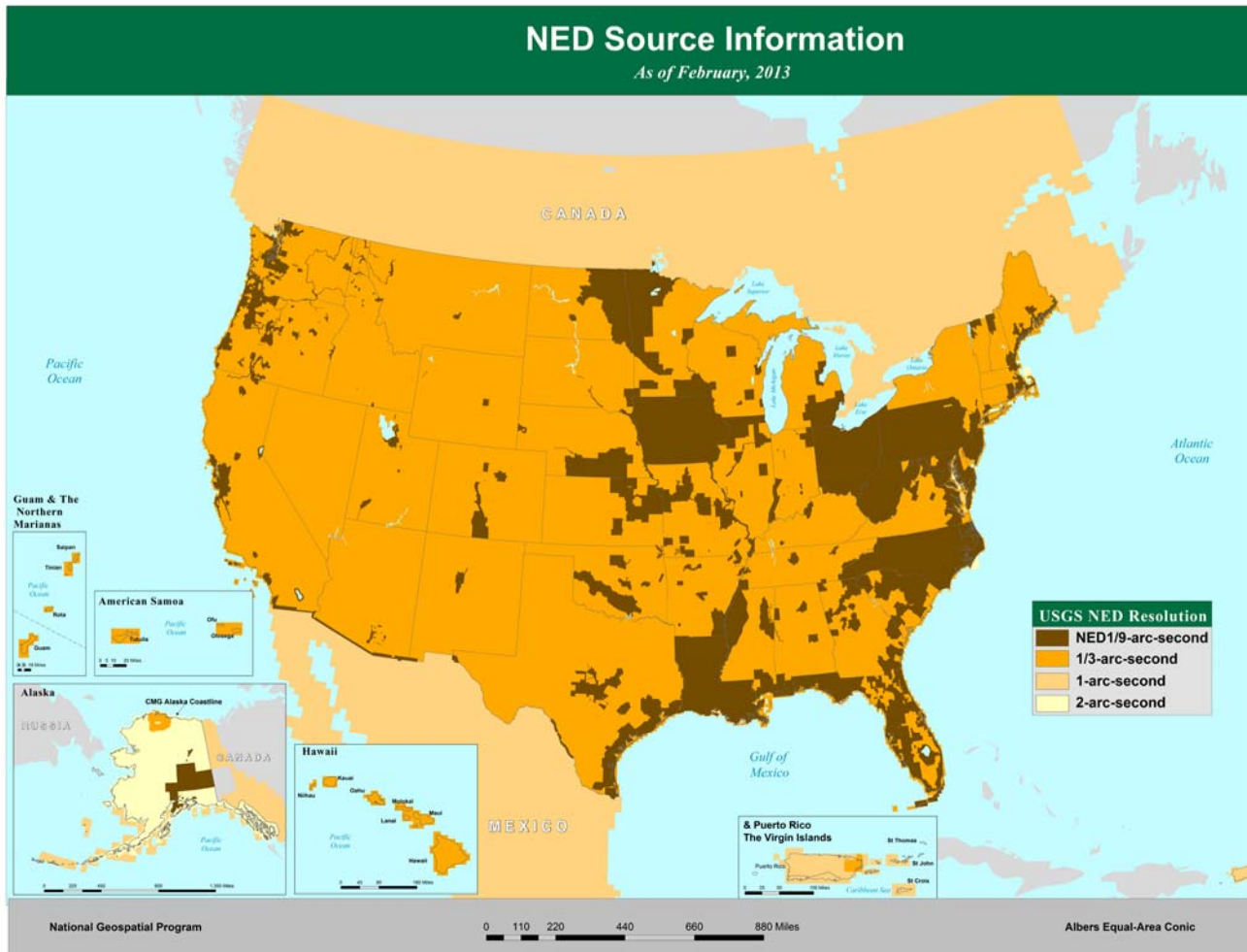
Figure 4. Composite of source data by resolution – February, 2013 release.
