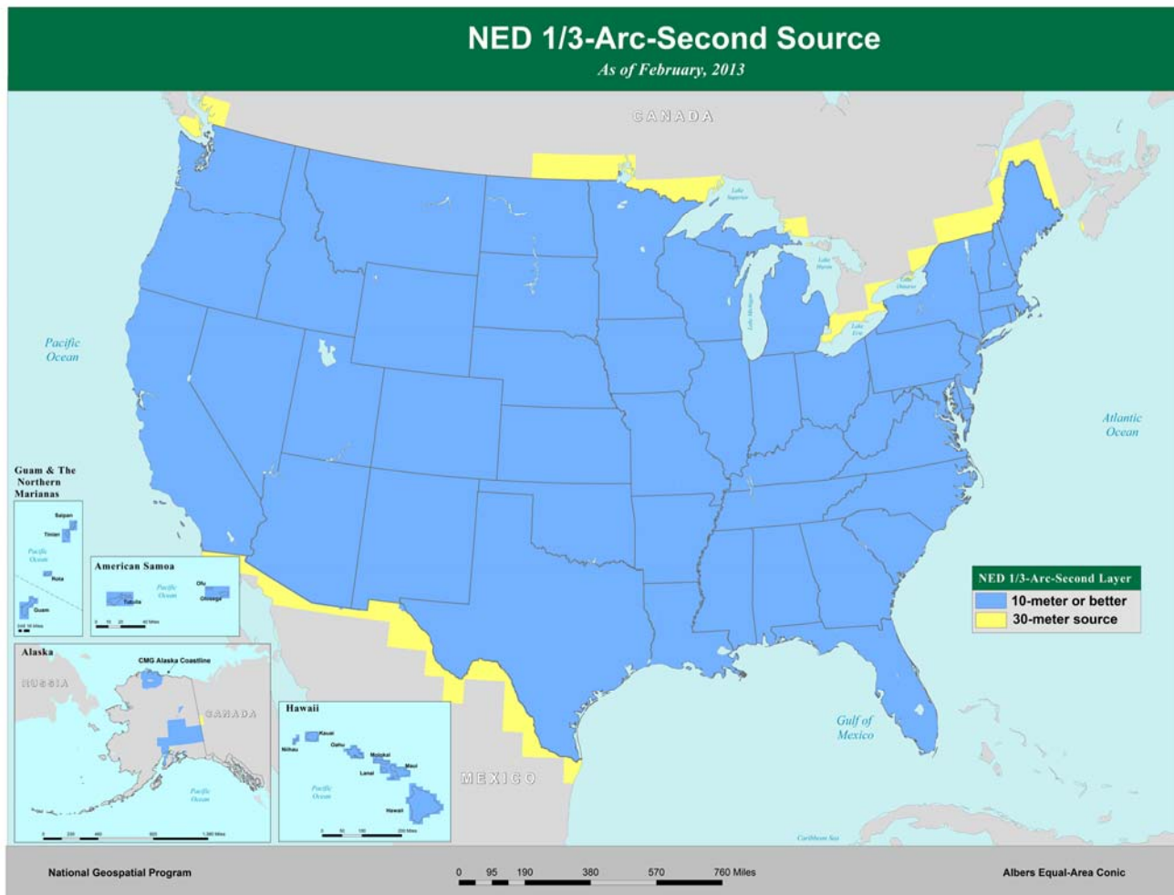
Figure 8. 1/3-arc-second NED, February, 2013 release by source resolution.
