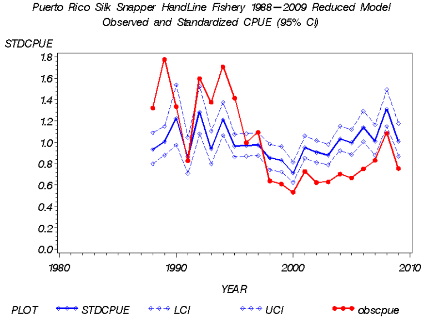
Figure 5. Standardized Delta –Lognormal CPUE, Upper and Lower 95% CI intervals and Nominal CPUE for silk Snapper handline fishery Base Run. (Figure 3.1.6.11 in the Assessment Workshop Report)
