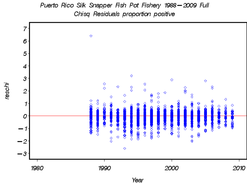
Figure 3.1.6.10. Residual distribution for binomial model fit to the silk snapper fish pot fishery data.
