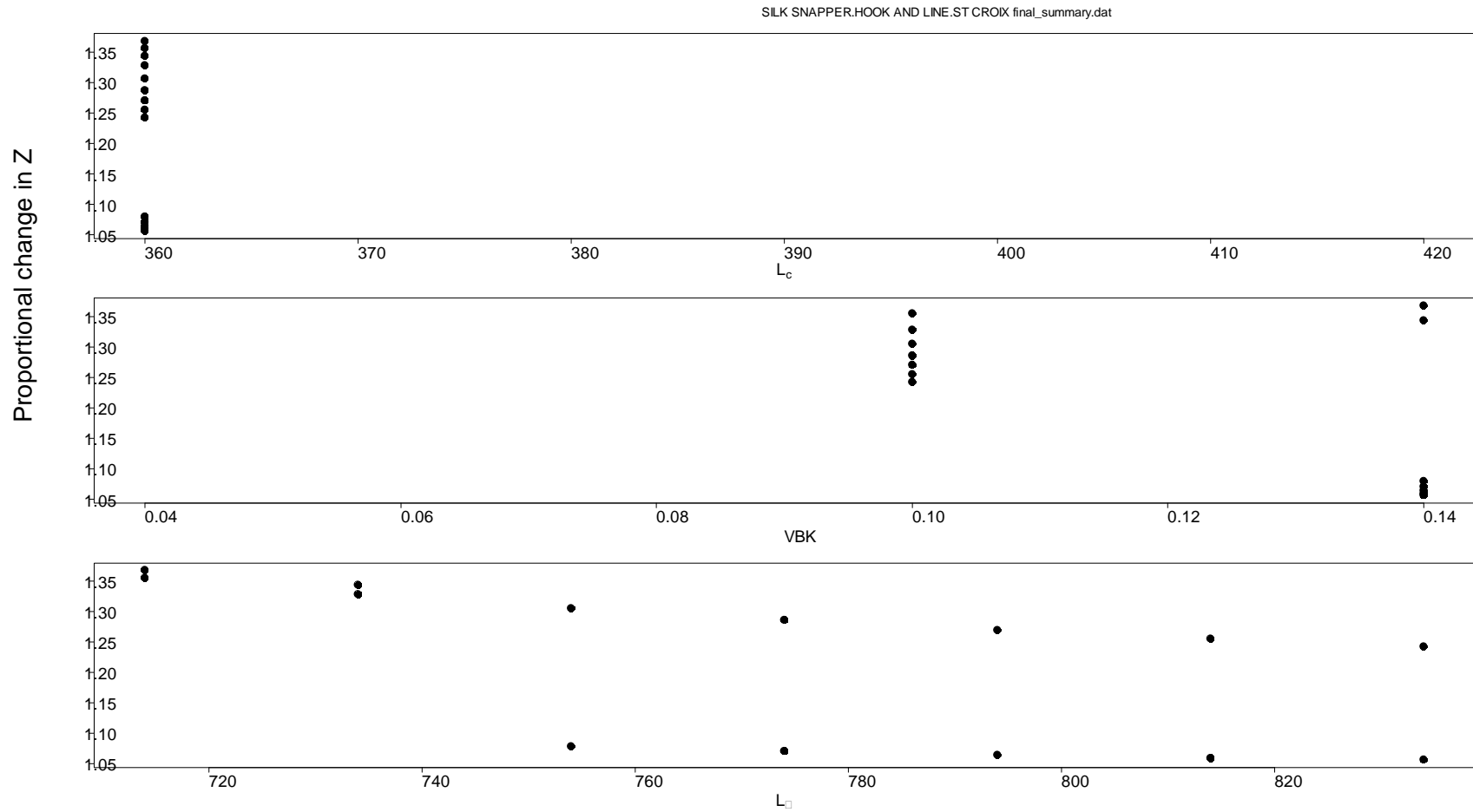
Figure 5.5.5. Proportion change in total mortality ( Z ) as a function of length at full vulnerability ( L_c ), the von Bertalanffy growth parameter (VBK) and asymptotic length ( L_\infty ) for Silk snapper caught by hook and line in St. Croix. Strong support \Delta AIC > 5 .
