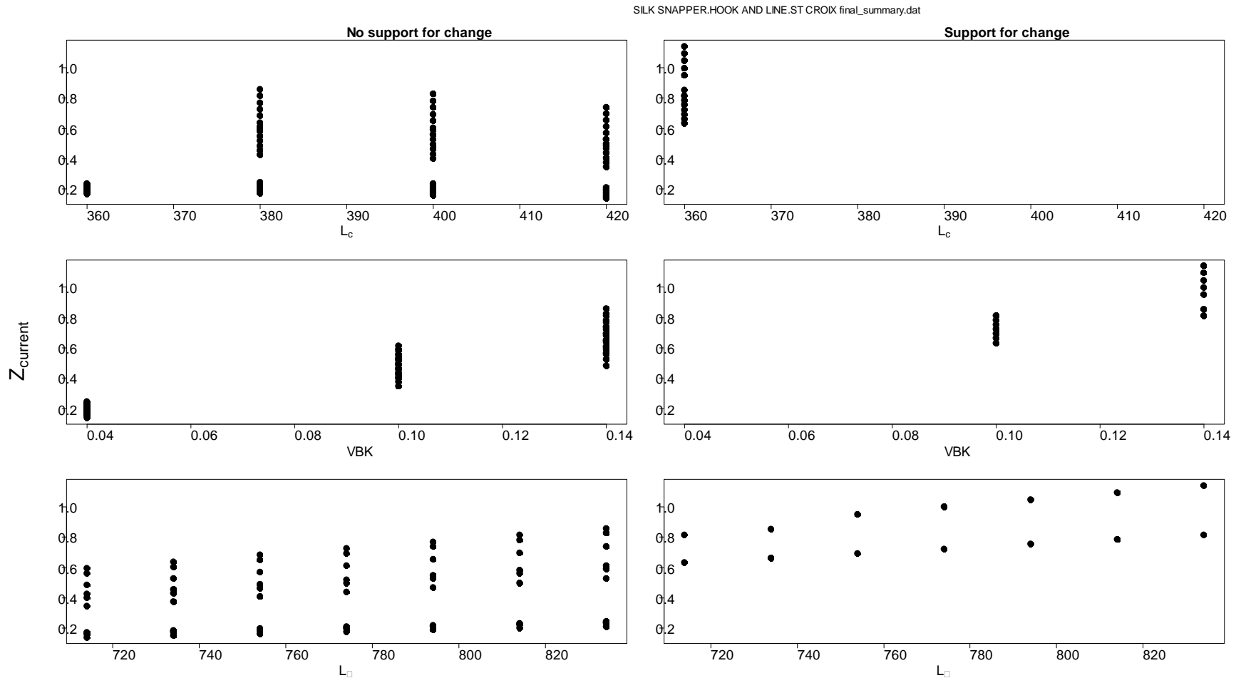
Figure 5.5.4. Current estimates of total mortality ( Z_{current} ) as a function of length at full vulnerability ( L_c , top panels), the von Bertalanffy growth parameter (VBK, middle panels), and asymptotic length ( L_\infty , bottom panels) when there was no support for change (left panels) and a support for change (right panels) from the time-series analysis for Silk snapper caught by hook and line in St. Croix. The base case parameter combination was 486mm for L_c , 0.1 for the von Bertalanffy growth parameter, and 794mm for L_\infty . Strong support \Delta AIC > 5 .
