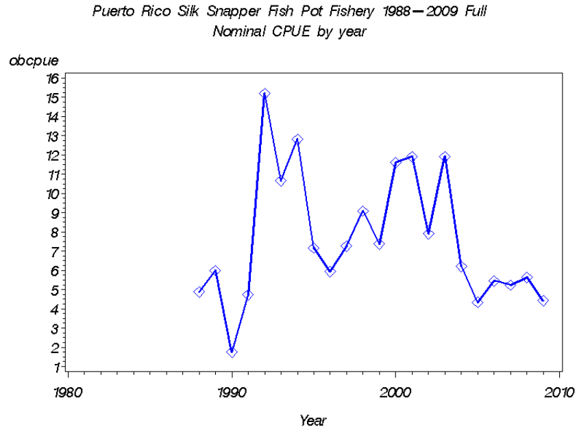
Figure 3.1.6.7. Nominal CPUE for silk snapper fish pot fishery.
