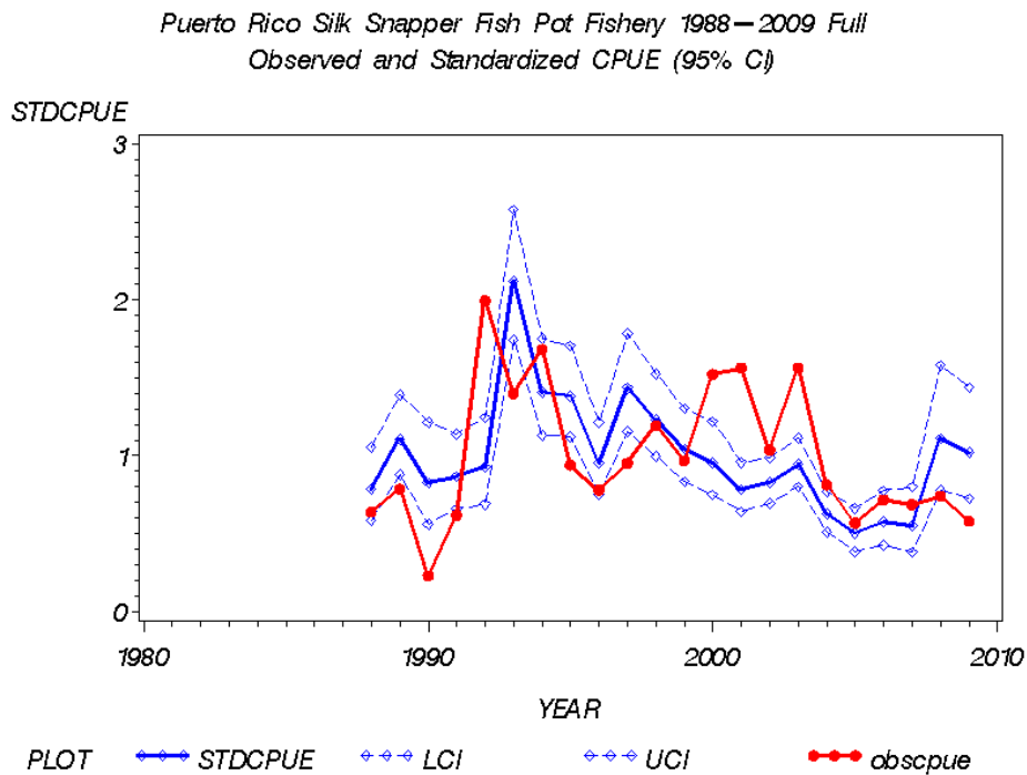
Figure 6. Standardized Delta –Lognormal CPUE, Upper and Lower 95% CI intervals and Nominal CPUE for Silk Snapper fish pot fishery Base Run. (Figure 3.1.6.15 in the Assessment Workshop Report)
