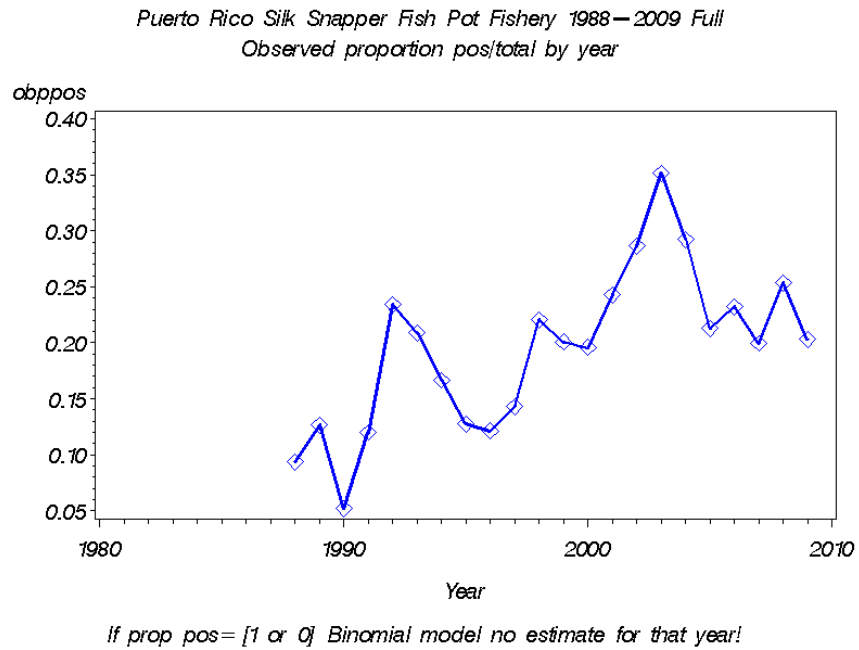
Figure 3.1.6.8. Proportion of Positives for silk snapper fish pot fishery.
