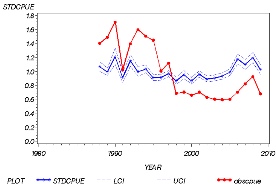
Figure 3.1.6.13. Standardized lognormal CPUE, Upper and Lower 95% CI intervals and Nominal CPUE for silk Snapper handline fishery 50% landing trip weight cutoff run.
