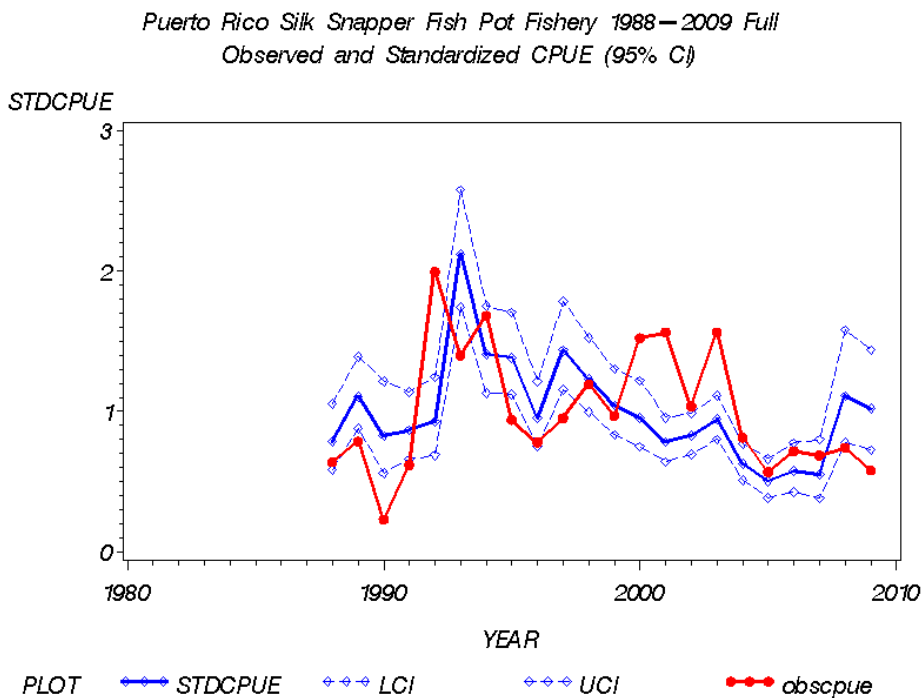
Figure 3.1.6.15. Standardized Delta –Lognormal CPUE, Upper and Lower 95% CI intervals and Nominal CPUE for silk Snapper fish pot fishery Base Run.
