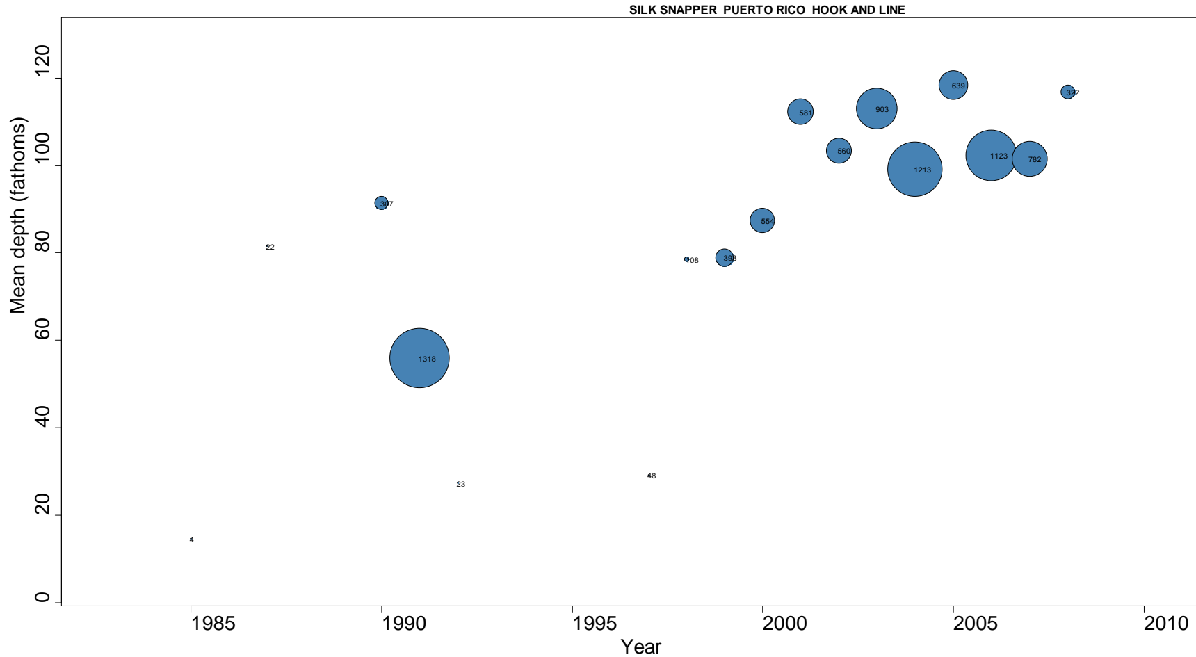
Figure 2.6.11. Mean depth (measured in fathoms) of fishing and capture of silk snapper by the hook and line fishery in Puerto Rico. Bubble size indicates the number of interviews from the TIP database for a given year that were used to calculate the mean and is scaled with respect to other years. The numbers plotted within the figure represent the number of interviews per bubble.
