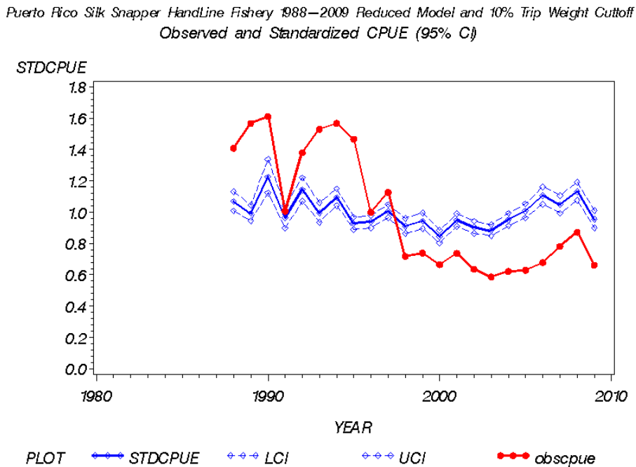
Figure 3.1.6.12. Standardized lognormal CPUE, Upper and Lower 95% CI intervals and Nominal CPUE for silk Snapper handline fishery 10% landing trip weight cutoff run.
