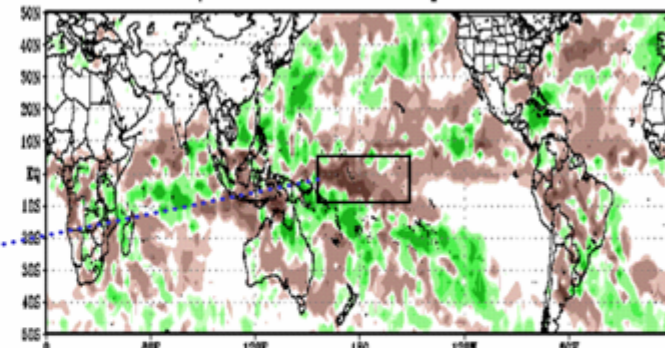
SSM/I Rainfall Anomaly Dec 2000
