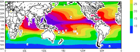
SSM/I TPW (1987-07) JUN, JUL, AUG
