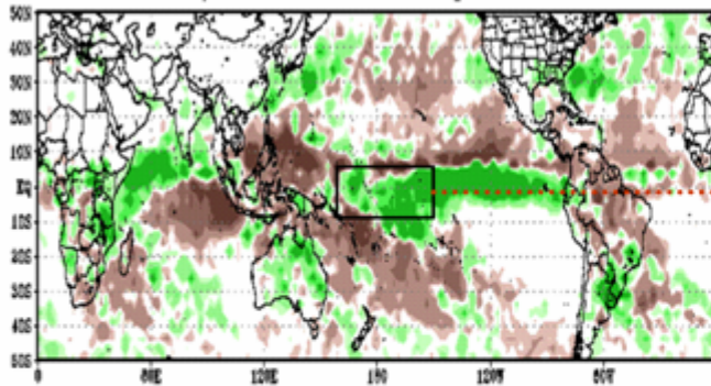
SSM/I Rainfall Anomaly Dec 1997
