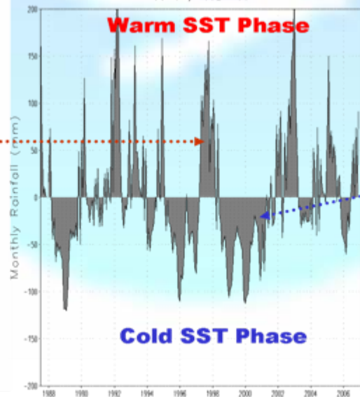
Nino4 Monthly Rainfall Anomaly (mm/mon) from SSM/I 5S-5N, 160E-150W
