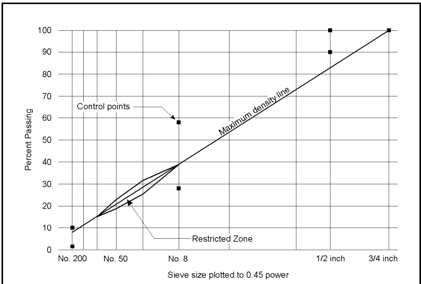
Figure 703-1 Gradation Chart for 0.5-Inch Nominal Maximum Size Aggregate
