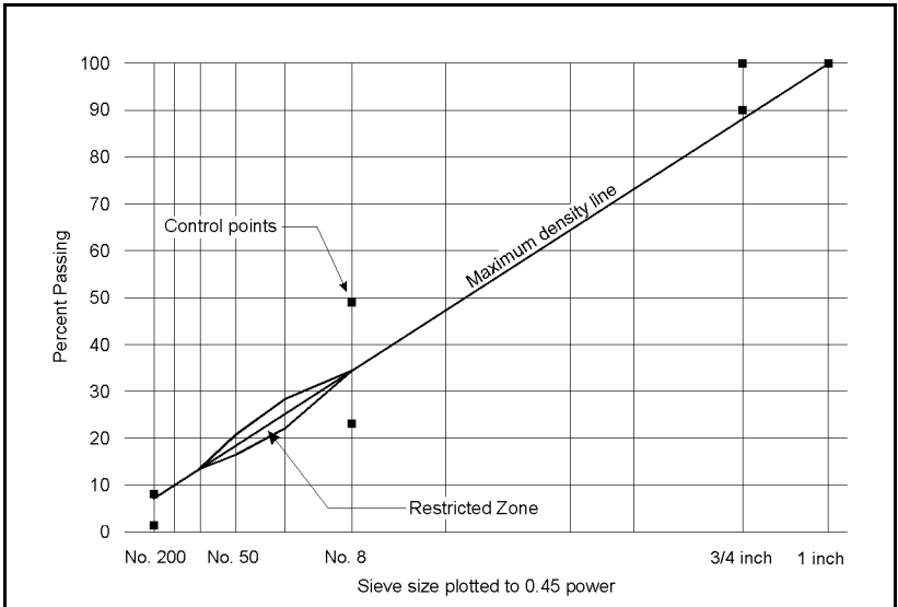
Figure 703-2 Gradation Chart for 0.75-Inch Nominal Maximum Size Aggregate
