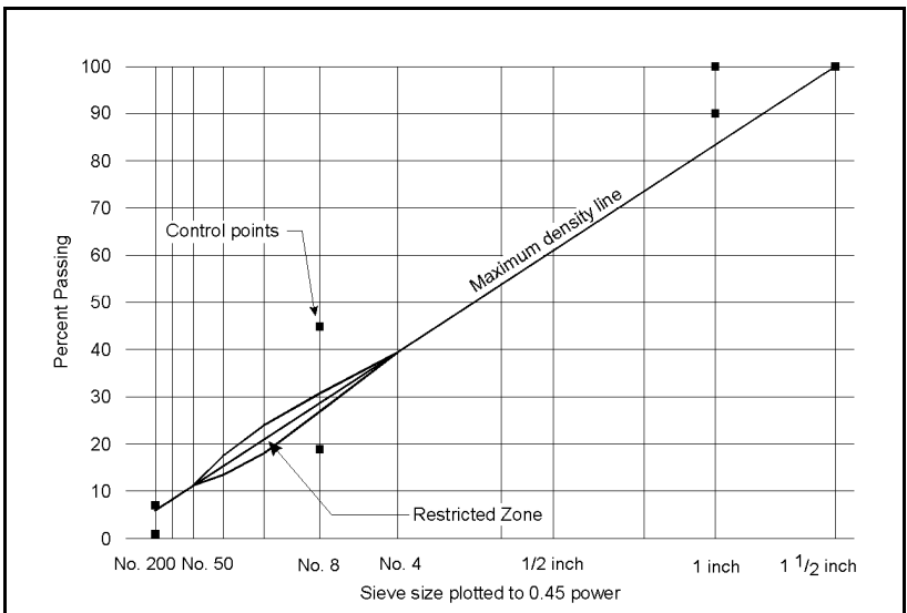
Figure 703-3 Gradation Chart for 1-Inch Nominal Maximum Size Aggregate
