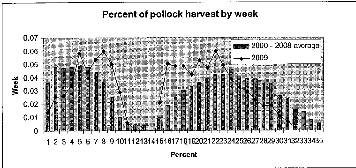
Figure 7. Percent of pollock catch by week.
