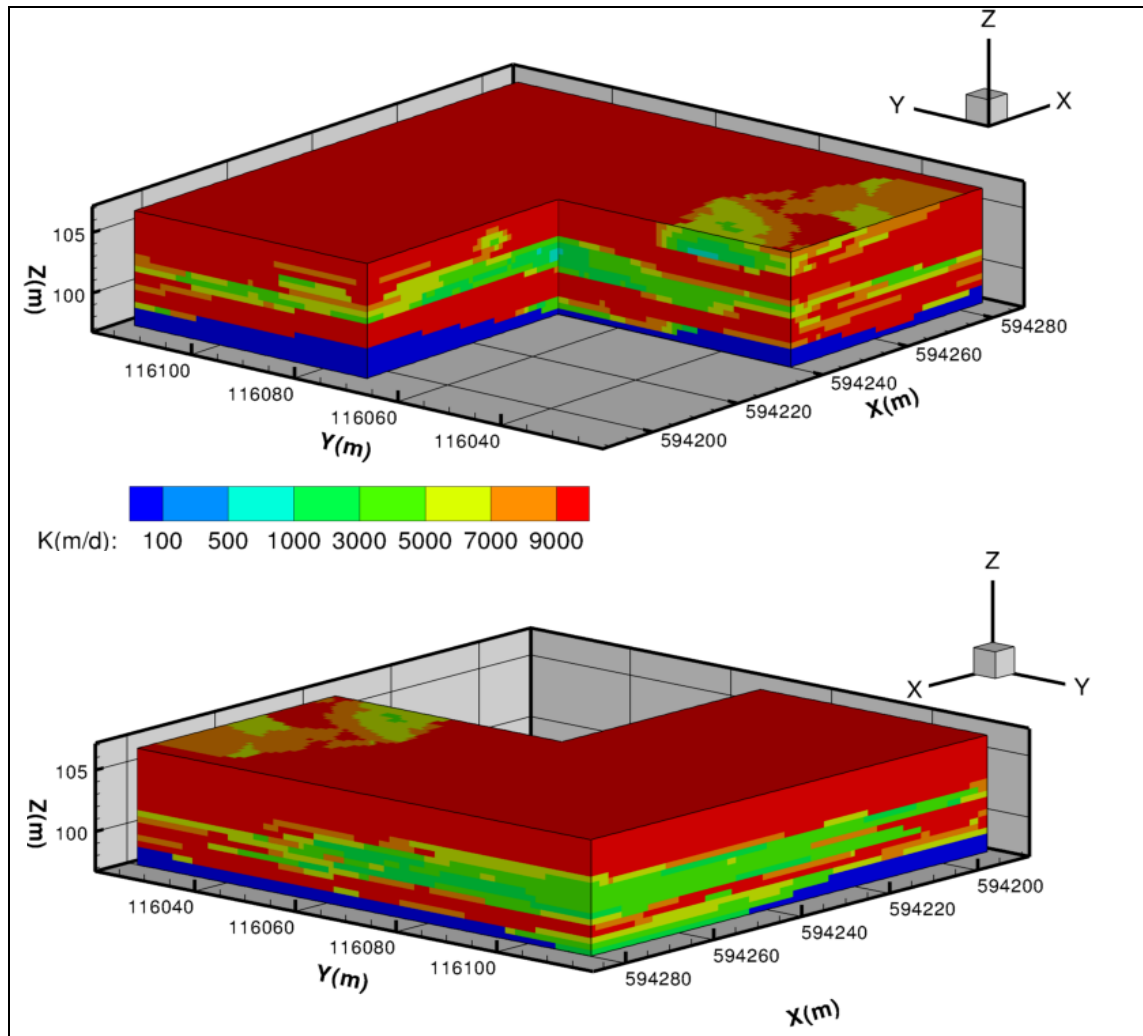
Figure 8. Cutaway views of an estimated hydraulic conductivity distribution at the Hanford 300 Area IFRC well field.
