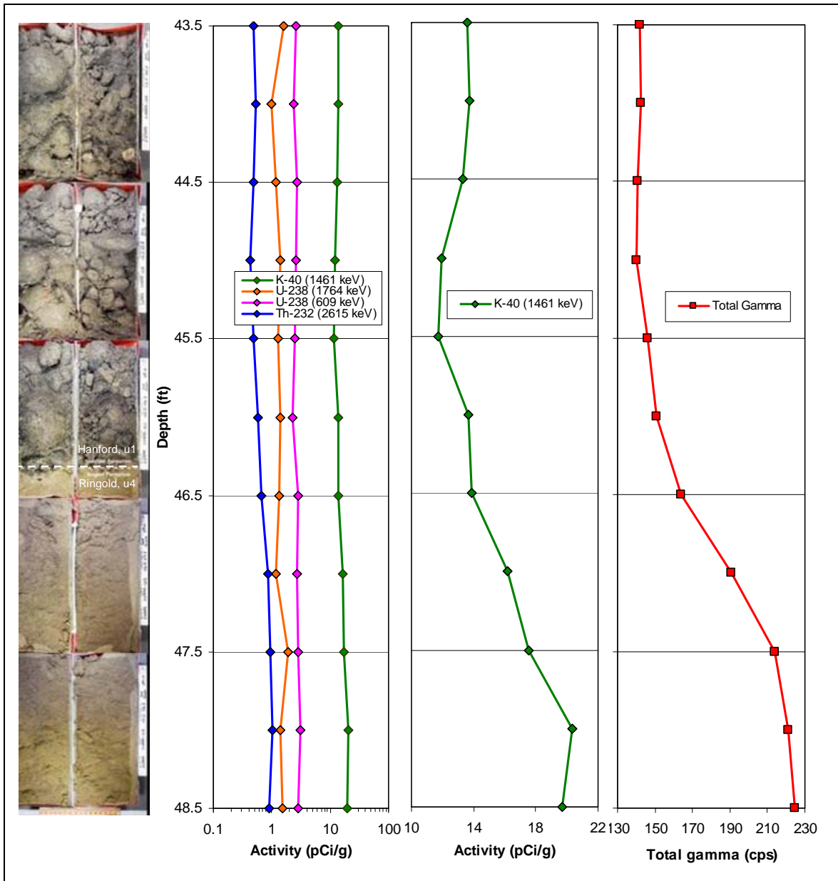
Figure 5. Split-core photographs of sediment samples from both the Hanford (upper 2 cores) and Ringold (lower 2 cores) Fm collected during drilling of well 399-3-18 (located ~200 m east of the IFRC well field), and spectral gamma and total gamma log readings for the same depth interval (from Williams et al, 2008). Note the differences in texture between the Hanford and Ringold Fm sediments, the sharp break between them, and the corresponding smoothly varying responses from the gamma logs across this interface.
