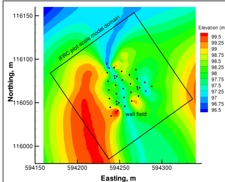
Figure 3. Map showing interpreted elevation of surface of Hanford-Ringold Fm contact in vicinity of Hanford 300 Area IFRC site. Black dots show well locations and black square shows approximate plan-view extent and orientation of numerical flow and transport models being applied to evaluate field experiments. Note apparent channel feature extending through center of well field.
