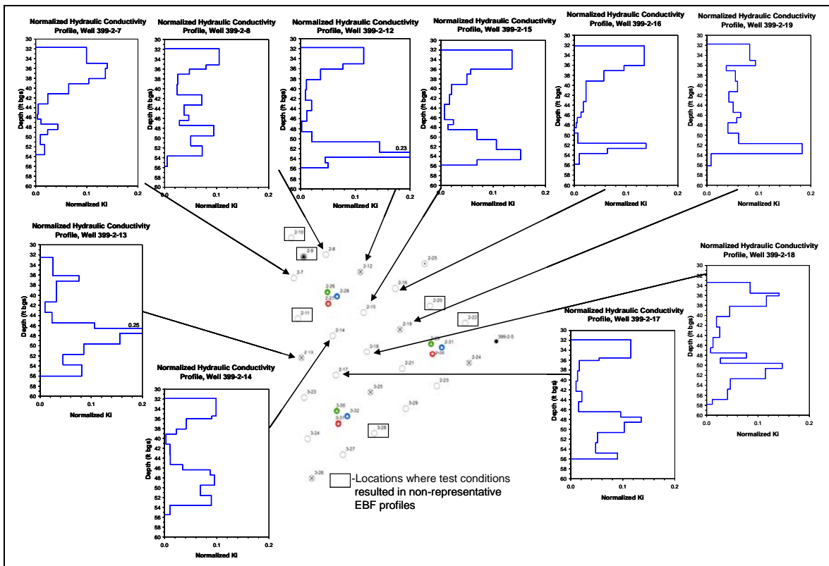
Figure 6. Normalized hydraulic conductivity profiles at selected Hanford 300 Area IFRC wells based on electromagnetic borehole flow meter testing.
