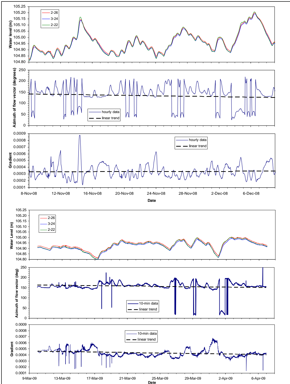
Figure 7. Observed water levels and computed flow directions and gradients during the November 2008 (top 3 panels) and March 2009 tracer tests (bottom 3 panels) at the Hanford 300 Area IFRC site. Note that the flow conditions were much more stable during the March 2009 test.
