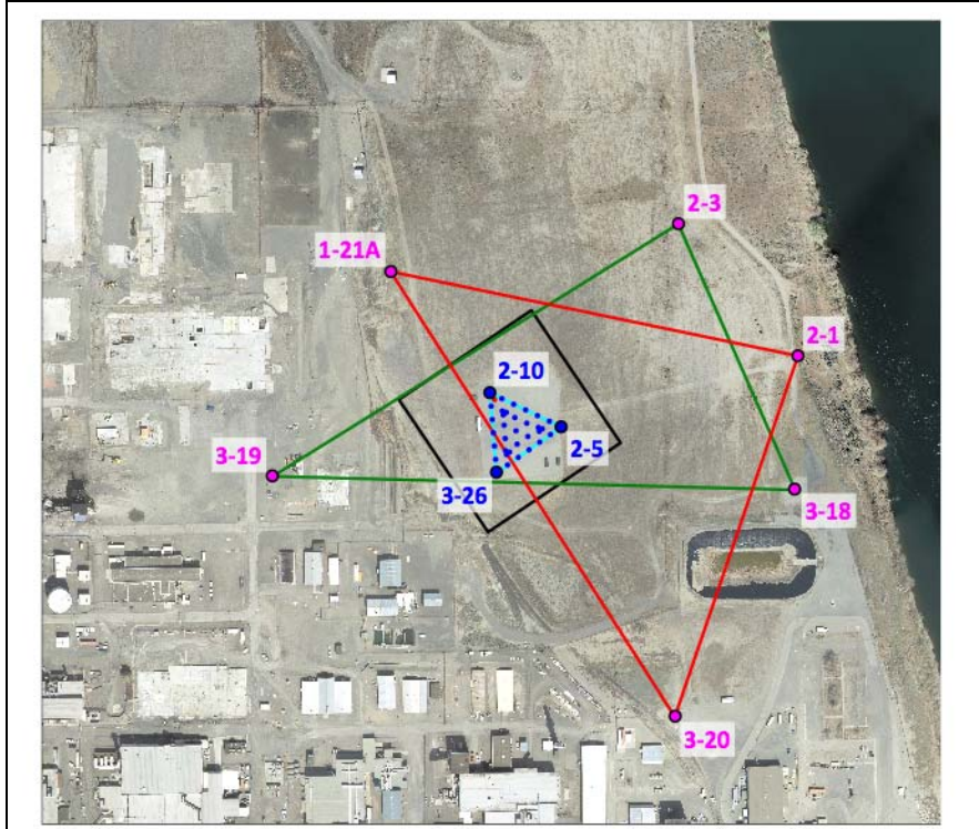
Figure V-11. Boundary conditions for scenarios A (green), B (red) and C (black).
