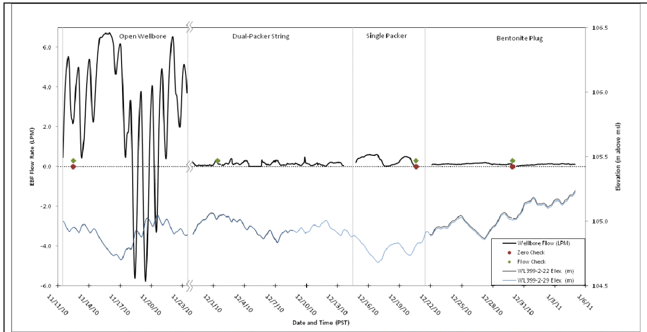
Figure II-5. Temporal trends in ambient vertical flows in test well 2-22 during the wellbore flow mitigation trials. Water-level elevation data are shown for comparison.
