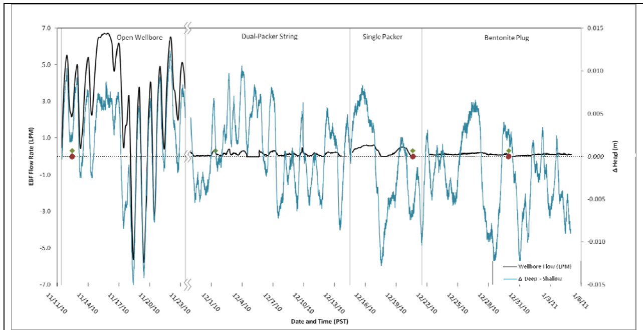
Figure II-6. Temporal trends in ambient vertical flows in test well 2-22 during the wellbore flow mitigation trials. Water-level elevation data are shown for comparison.
