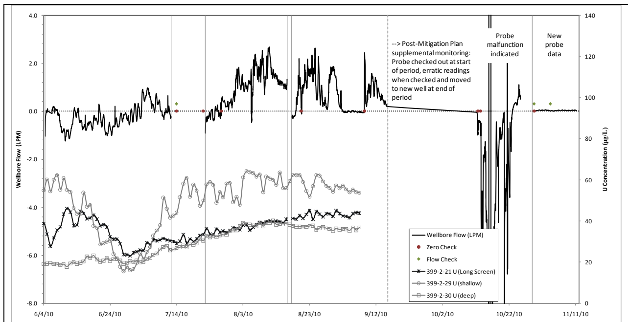
Figure II-3. Temporal trends in U concentration and ambient vertical flows in test well 2-21 during the wellbore flow mitigation trials.
