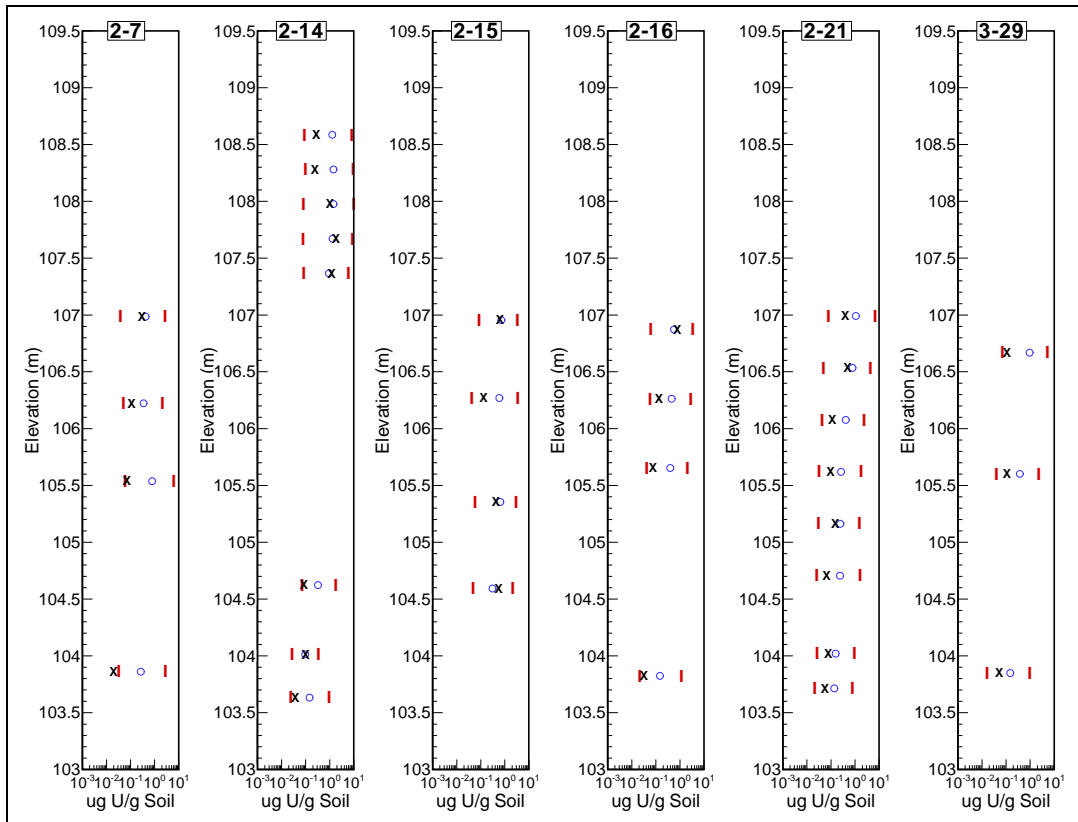
Figure III-13. Plots of predicted BEU versus measured values for samples from several wells where additional samples were measured in CY 2010. The blue circles are the predicted means, x's represent the measured values, and the red bars represent a 95% confidence interval for each prediction.
