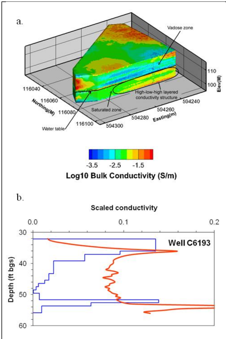
Figure III-2. a) Section of 3D ERT inversion results showing the estimated bulk conductivity structure within the IFRC well-field. The saturated zone displays a layered bulk conductivity structure that may be well correlated to permeability as shown in b. b) Comparison of scaled hydraulic conductivity (blue) and scaled bulk conductivity (red) extracted from the ERT inversion results at one IFRC well, demonstrating a possible correlation between bulk conductivity and permeability within the saturated zone. Other wells display similar correlations.
