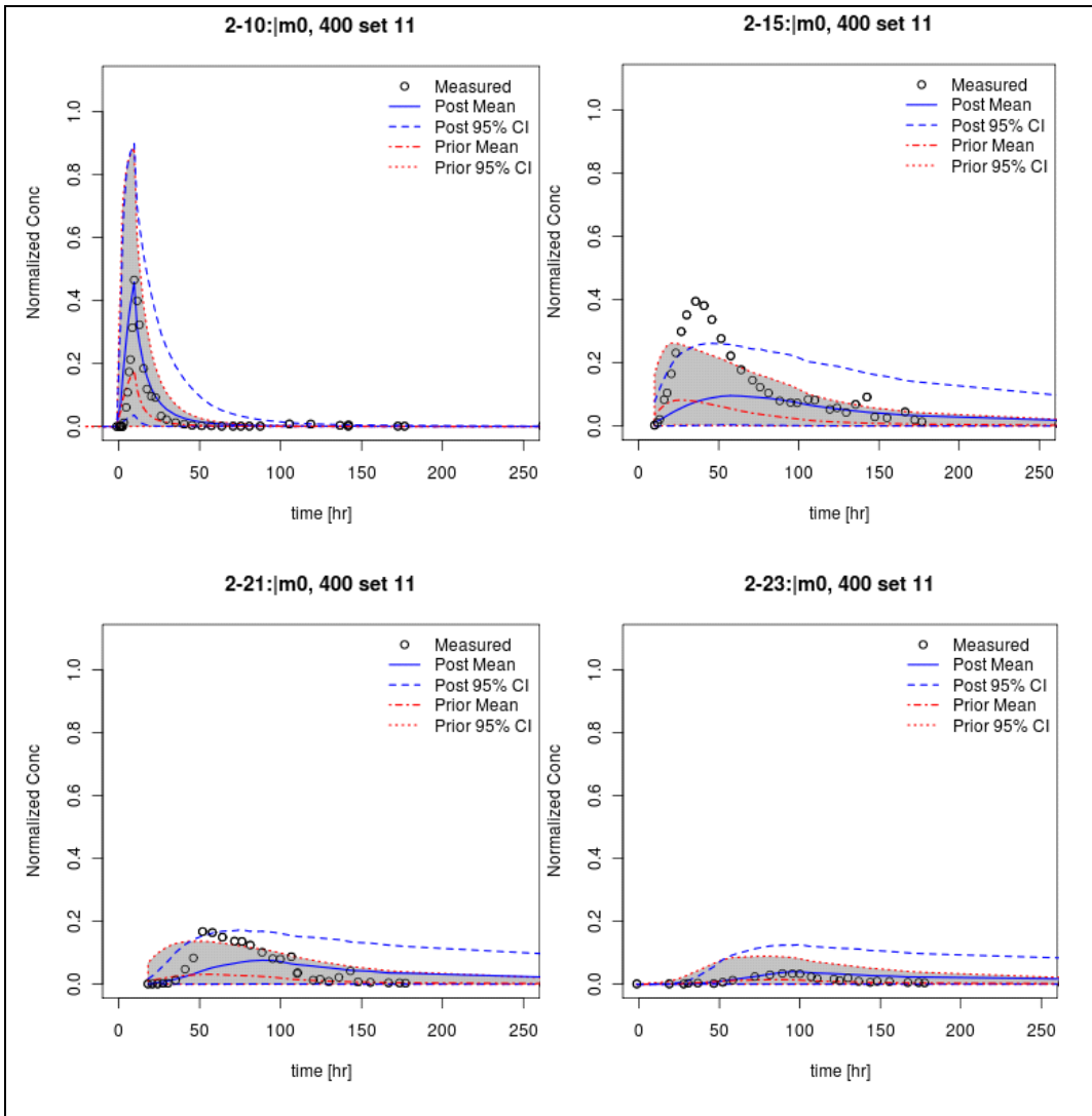
Figure III-1. Validation of breakthrough curves in selected wells for Mar09 Tracer Test (from Chen et al., 2011).
