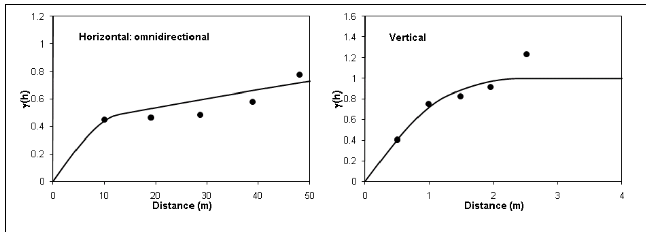
Figure III-7. Horizontal and vertical variograms of the BEU normal scores. The normal scores were calculated on the raw data, not gravel corrected. Black dots represent variogram values calculated from the data, and solid black line represents the model fit.
