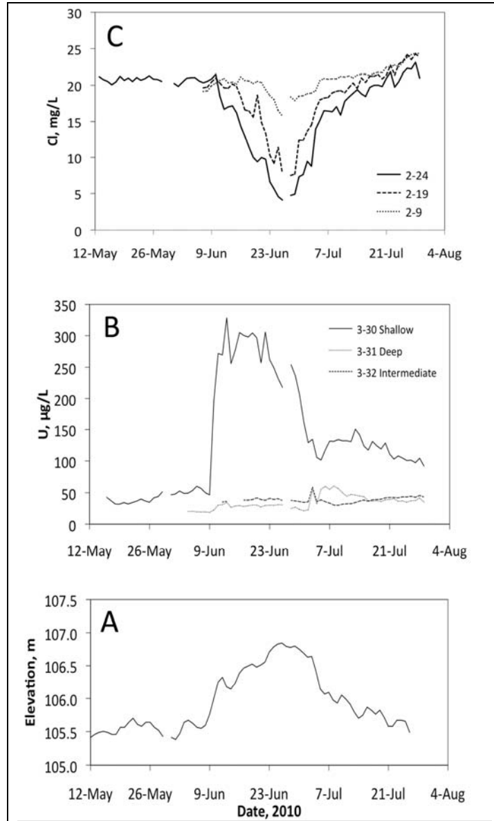
Figure IV-1. Selected time series groundwater data, collected during major spring-melt water table excursions. A) Water table elevation; B) U concentrations at the south corner of the IFRC, for the shallow, intermediate and deep portions of the unconfined aquifer; and C) Cl - concentrations for three wells that transect the IFRC from east to north.
