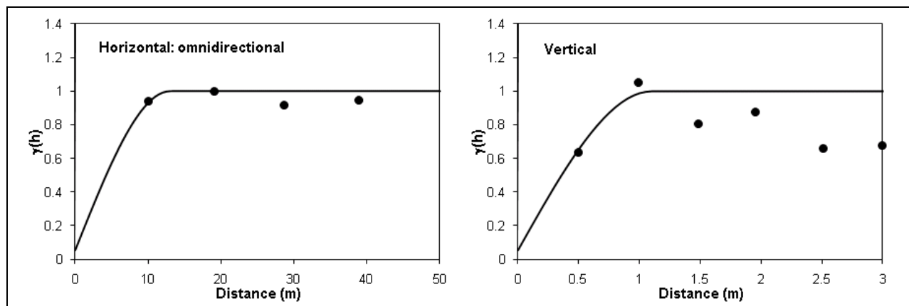
Figure III-11. Experimental variograms and models for K_d for U-233. The normal scores were calculated on the raw data, not gravel corrected. Black dots represent variogram values calculated from the data, and solid black line represents the model fit.
