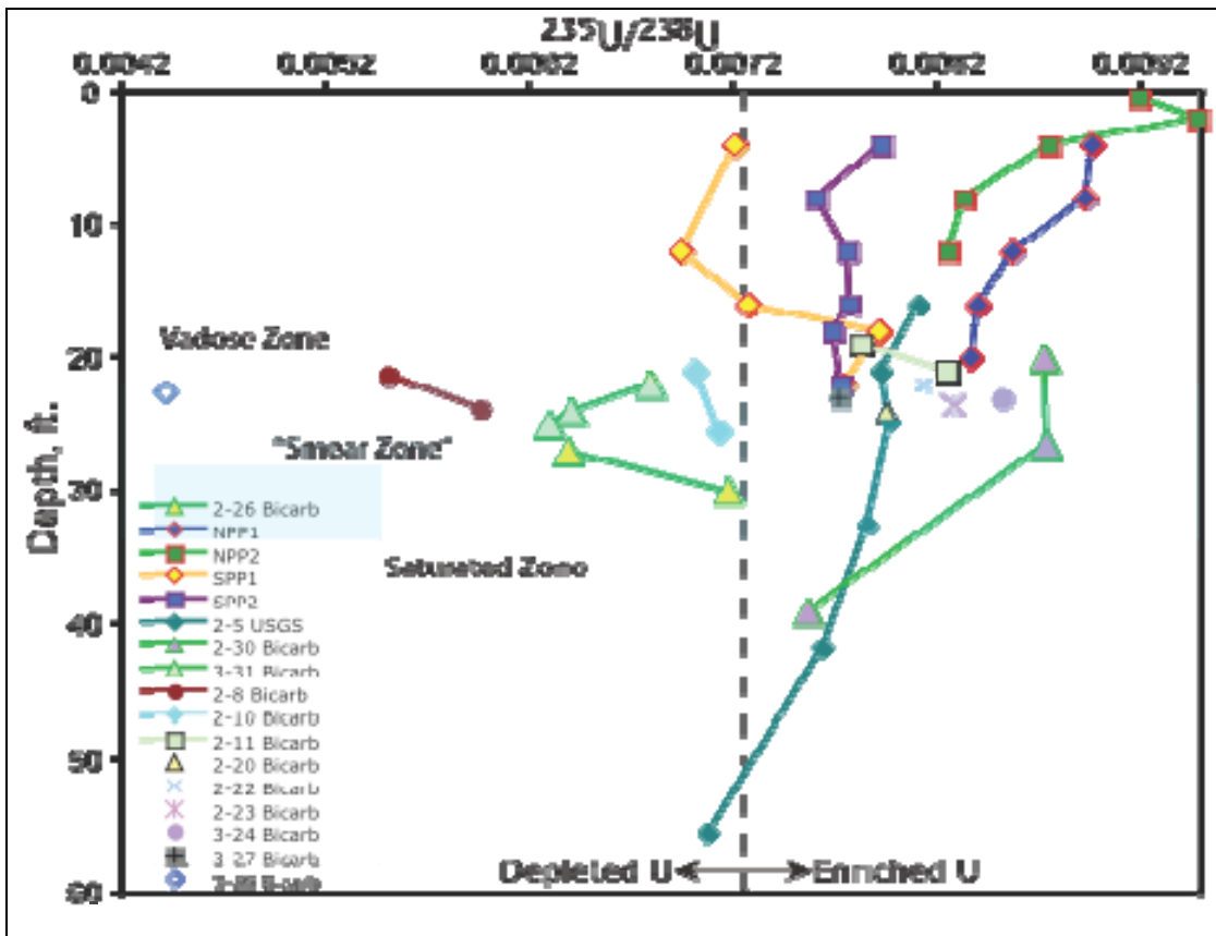
Figure IV-3. Plot of ^{235}\text{U}/^{238}\text{U} of sediment sample leachates vs. sampling depth. Significant U isotopic local spatial heterogeneity (vertical & horizontal) is represented by the sampled IFRC sediments, including within the "smear" zone.
