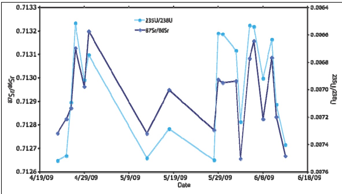
Figure IV-5. Time series comparing ^{87}\text{Sr}/^{86}\text{Sr} and ^{235}\text{U}/^{238}\text{U} (shown in reverse scale) for well 3-30.
