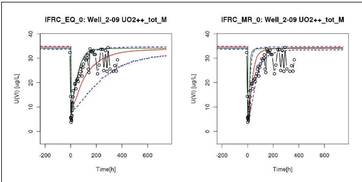
Figure V-14. Comparison of model simulations for U(VI) concentration with field data for boundary condition scenario C.
