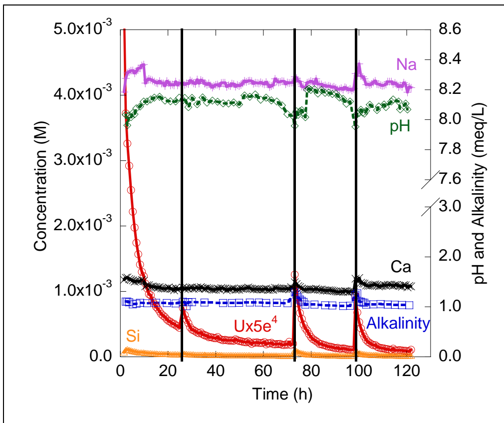
Figure V-2. Aqueous chemical conditions observed during a flow-through batch extraction with SWC <2 mm in an AGW with 1 meq/L alkalinity, at 100 g/L, 20 mL/h. Black lines represent stop flow events of 2.5h, 96h and 141 h duration.
