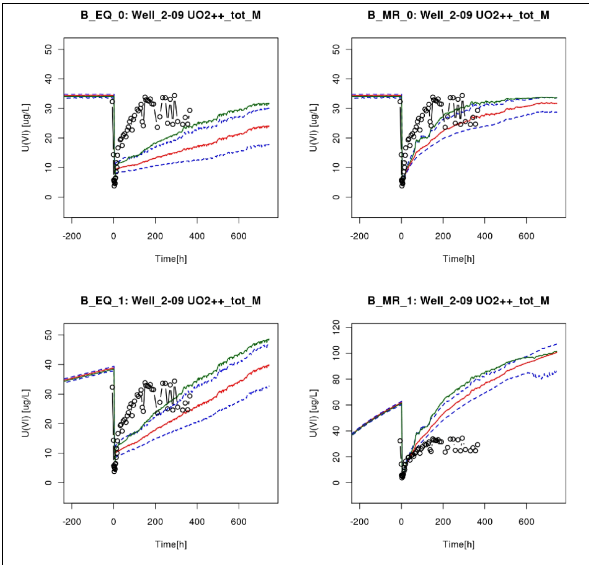
Figure V-13. Comparison of model simulations for U(VI) concentration with field data for boundary condition scenario B.
