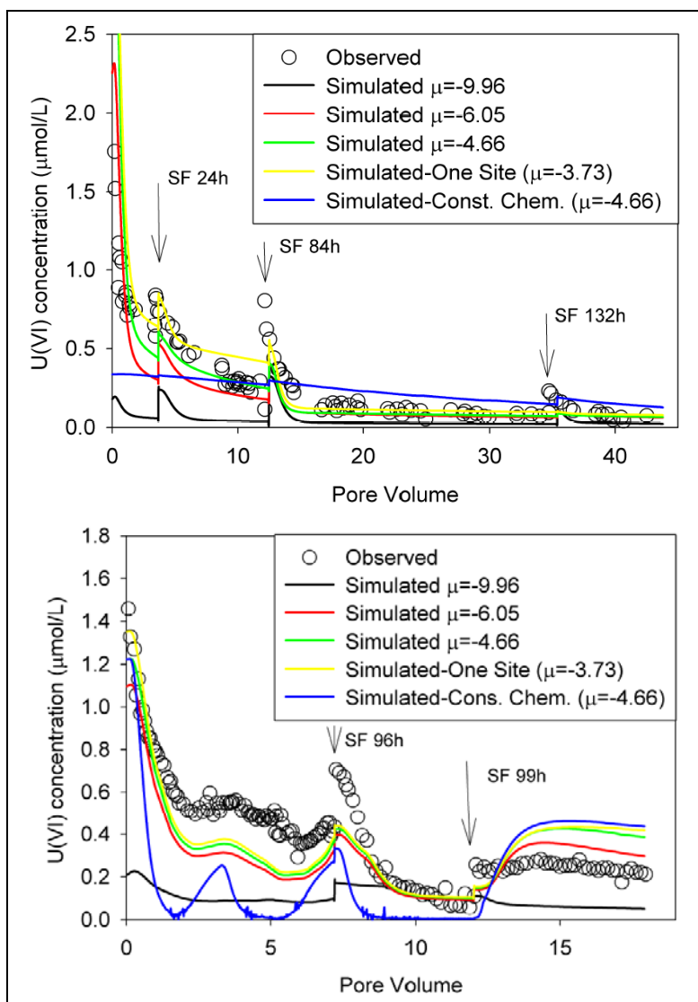
Figure V-7. Transient water chemistry. Observed and simulated U(VI) desorption in Experiment set 1: a) desorption (column #1); b) transient chemistry desorption (column #2).
