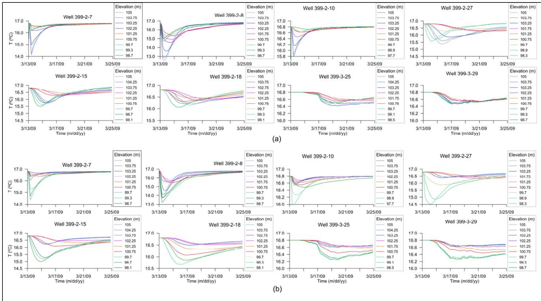
Figure V-10. Simulated temperature breakthrough curves at different depths of each observation well without (a) and with (b) consideration of the fluid density effect.
