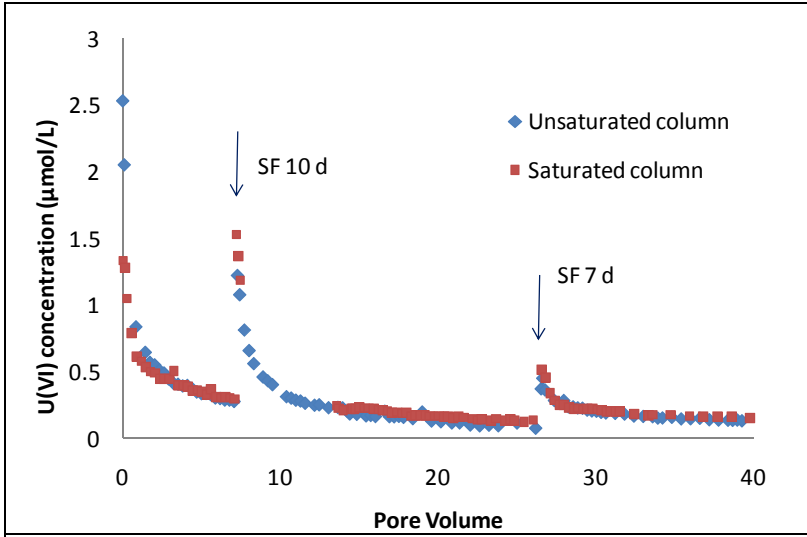
Figure V-8. Observed U(VI) concentrations in the transient water table experiment. During the stop flow events, one of the columns was allowed to drain (unsaturated) while the other was kept fully saturated. The pore volume needed to re-saturate the unsaturated column is not included in the calculation of pore volumes.
