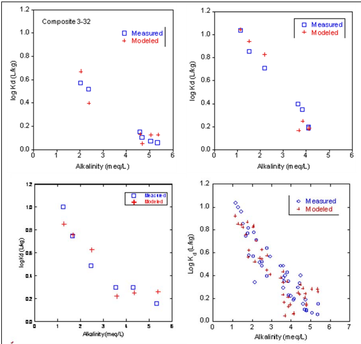
Figure V-1. Equilibrium U(VI) adsorption, expressed as the ratio of adsorbed (moles/kg) and dissolved (moles/L) U(VI) concentrations, on IFRC composites 3-32 (lowest adsorption equilibrium constant), 2-31 (highest equilibrium constant), site-wide composite, and all samples. Model-calculated U(VI) adsorption used the best-fit SCM for IFRC composites (reaction 1). Data from Yin et al., (in press) and Stoliker et al. (submitted).
