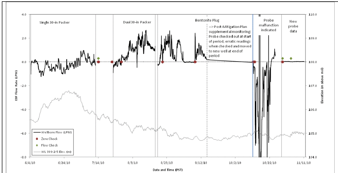
Figure II-2. Temporal trends in ambient vertical flows in test well 2-21 during the wellbore flow mitigation trials. Water-level elevation data are shown for comparison. EBF data collected from early August through October, when a defect in the probe cable was identified and the cable replaced, are spurious and should be disregarded.
