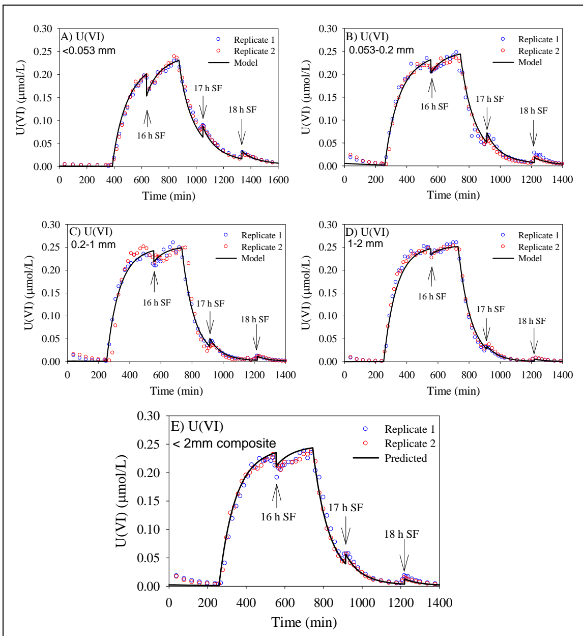
Figure V-5. Effluent U(VI) concentration profiles in different size fractions (A to D) and in composite (E). Circles are measured and lines are model-calculated results. The line in E was calculated by linearly adding the kinetic expressions for all size fractions weighted by their mass percentages in the sediment (composite).
