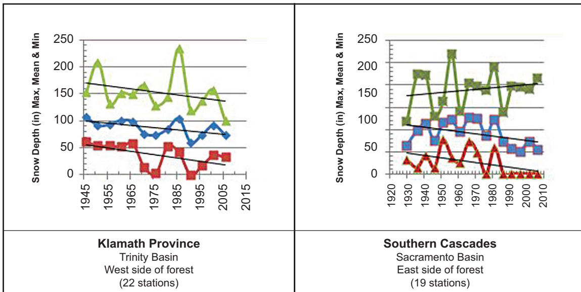
Figure 6. Changes in average snow depths from snow courses located in the Trinity River basin (1945-2009) and Sacramento River basin (1930-2009). Blue is the mean, red is the minimum, and green is the maximum snow depth.
