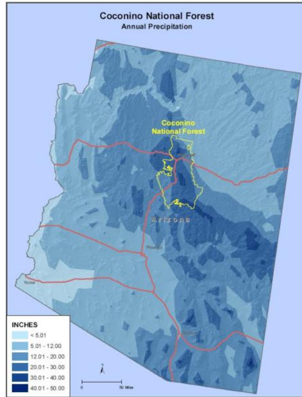
Figure 3. Annual precipitation for Arizona. Coconino NF and selected assessment watersheds include areas of relatively high precipitation for the region (from NOAA, 1994).
