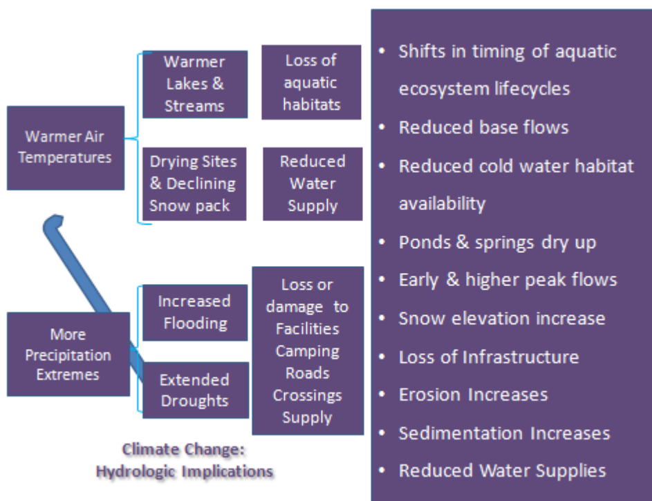
Figure 12. Summary of likely climate change effects on hydrologic processes, and on selected resource values
