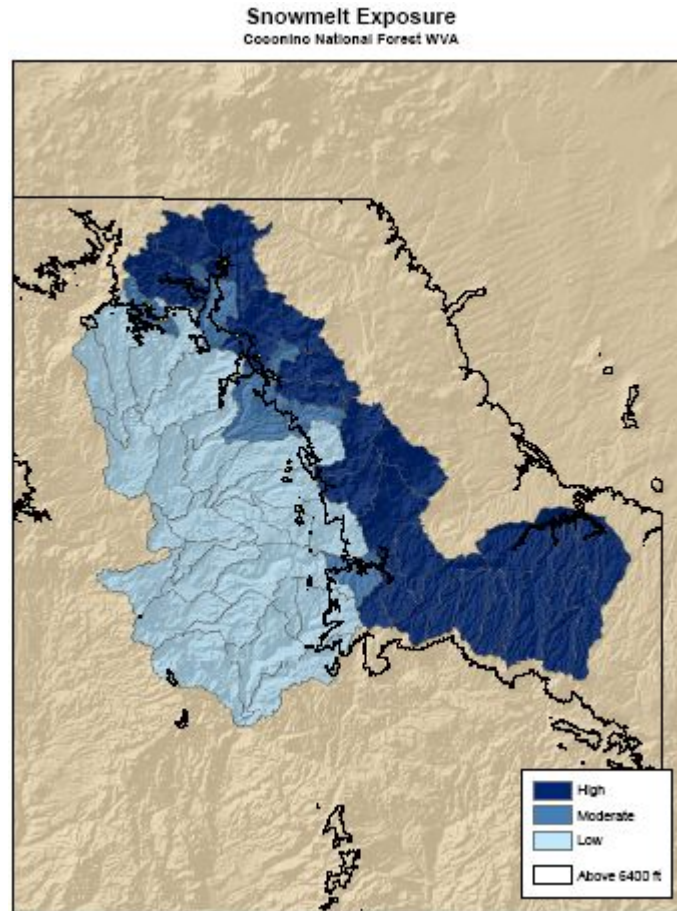
Figure 20. Relative exposure to potential climate change effects, based on % of subwatershed above 6400 ft
