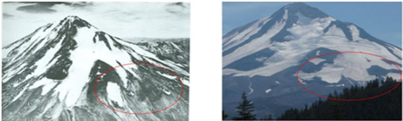
Figure 8. Photographs of the Hotlum Glacier, Mount Shasta, taken September 18, 1935 (left) and August 24, 2008 (right). Photos courtesy of Mount Shasta Climbing Rangers.
